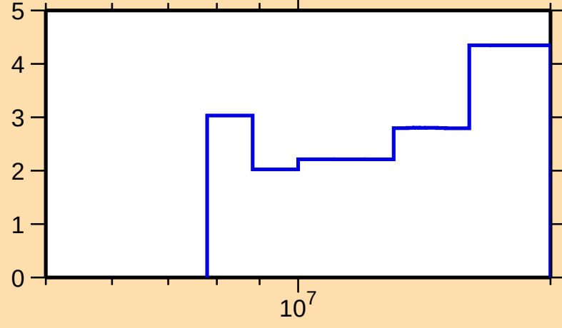
\Delta\sigma/\sigma vs. E for ^{115}\text{Te}(n,\text{tot.})
