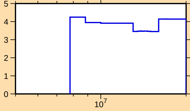
\Delta\sigma/\sigma vs. E for ^{115}\text{Te}(n,\text{nonel.})
