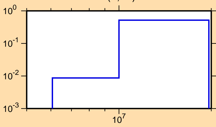
\sigma vs. E for ^{115}\text{Te}(n,2n)
