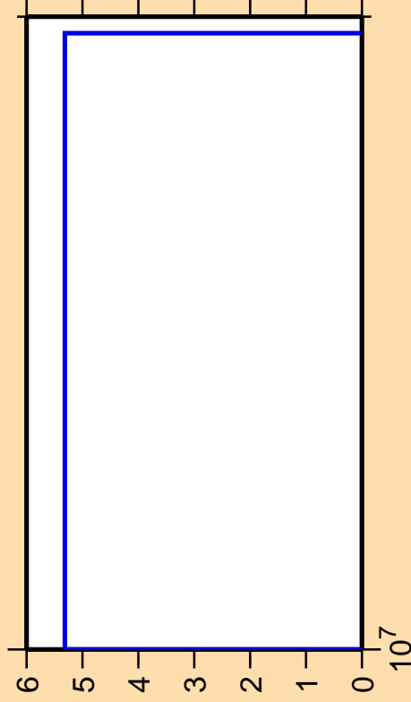
\Delta\sigma/\sigma vs. E for ^{115}\text{Te}(n,nt)
