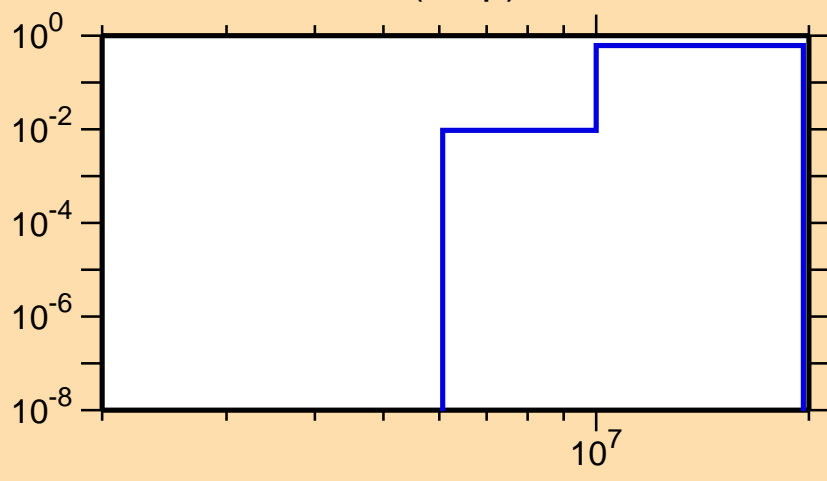
\sigma vs. E for ^{115}\text{Te}(n,np)
