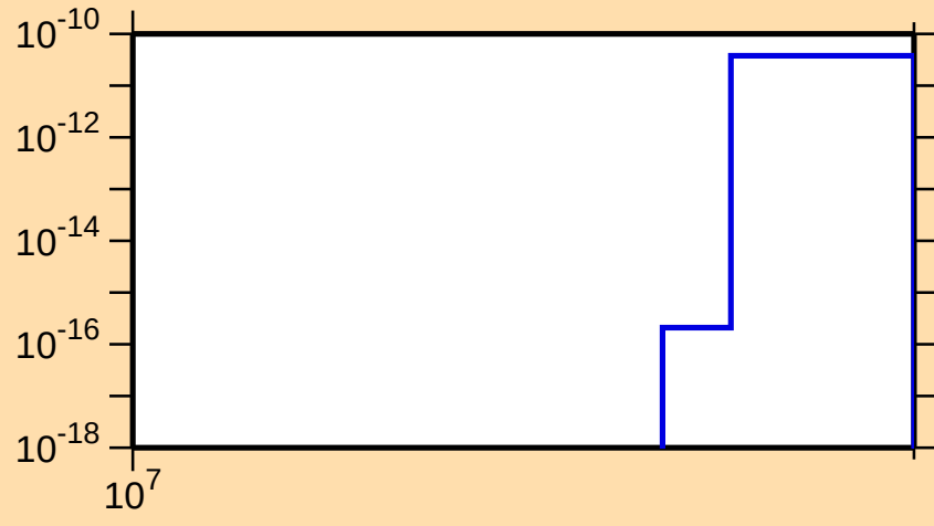
\sigma vs. E for ^{116}\text{Te}(n,\text{nt})
