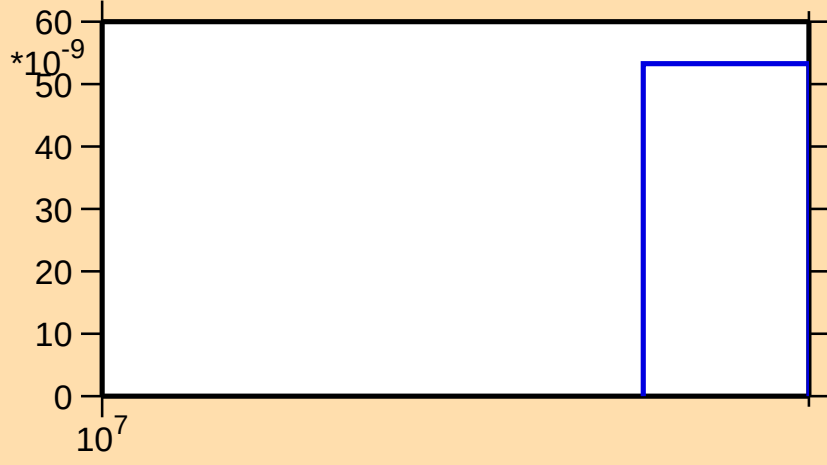
\sigma vs. E for ^{116}\text{Te}(n,3n)
