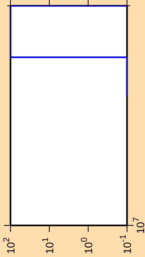
\Delta\sigma/\sigma vs. E for ^{116}\text{Te}(n,\text{nt})
