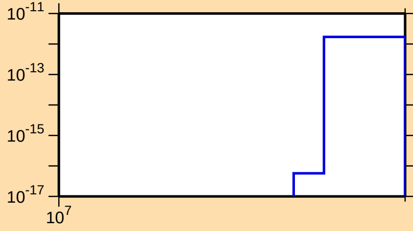
\sigma vs. E for ^{123}\text{Te}(n,\text{pt})
