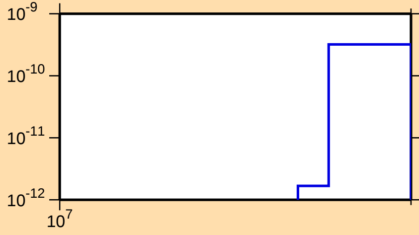
\sigma vs. E for ^{126}\text{Te}(n,\text{He3})
