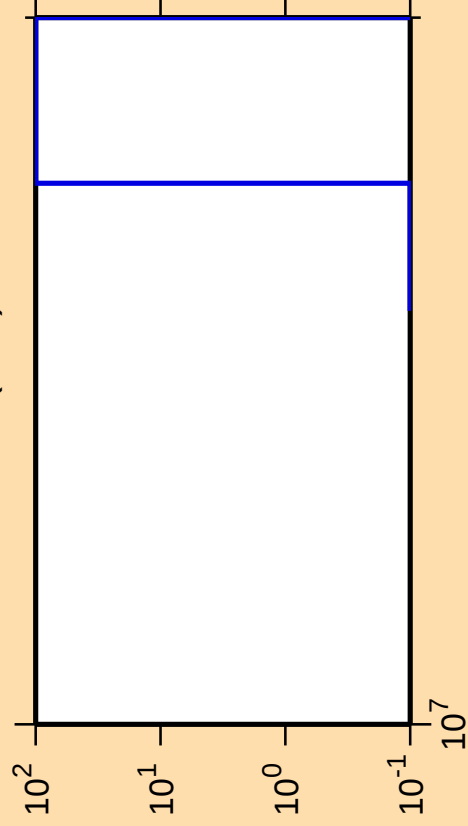
\Delta\sigma/\sigma vs. E for ^{126}\text{Te}(n,\text{nt})
