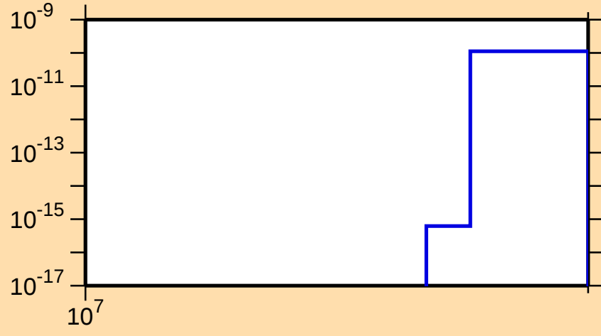
\sigma vs. E for ^{126}\text{Te}(n,\text{nt})
