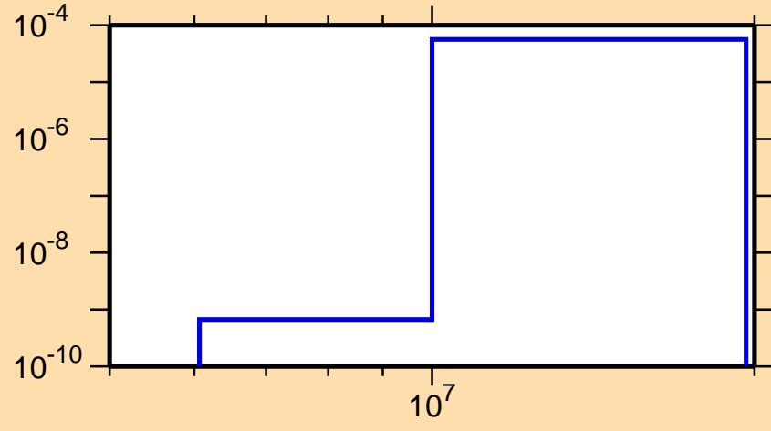
\sigma vs. E for ^{126}\text{Te}(n,\alpha)
