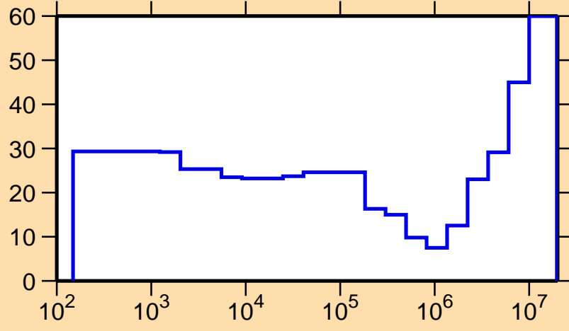
\Delta\sigma/\sigma vs. E for ^{127}\text{Te}(n,n_1)
