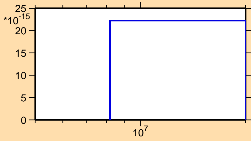
\sigma vs. E for ^{129}\text{Te}(n,\text{He3})
