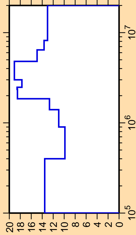
\Delta\sigma/\sigma vs. E for ^{129}\text{Te}(n,n_4)
