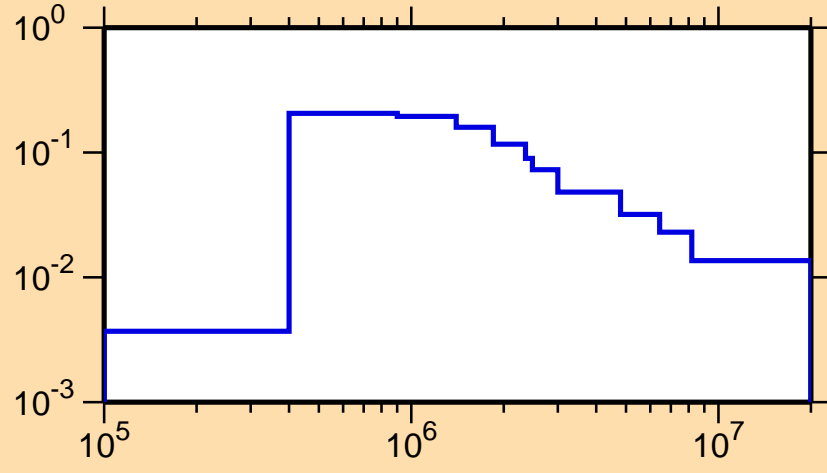
\sigma vs. E for ^{129}\text{Te}(n,n_4)
