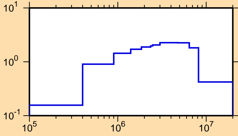
\sigma vs. E for ^{129}\text{Te}(n,\text{inel.})
