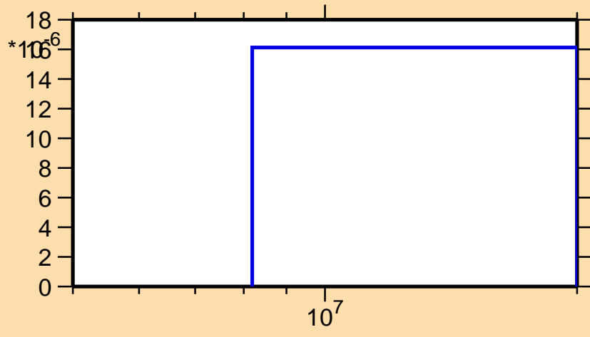
\sigma vs. E for ^{129}\text{Te}(n,n\alpha)
