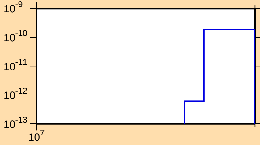
\sigma vs. E for ^{133}\text{Te}(n,2n\alpha)
