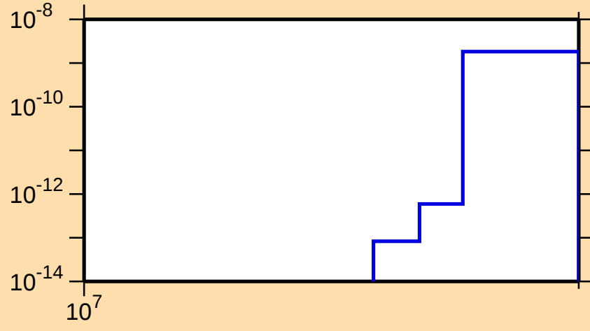
\sigma vs. E for ^{133}\text{Te}(n,\text{nt})
