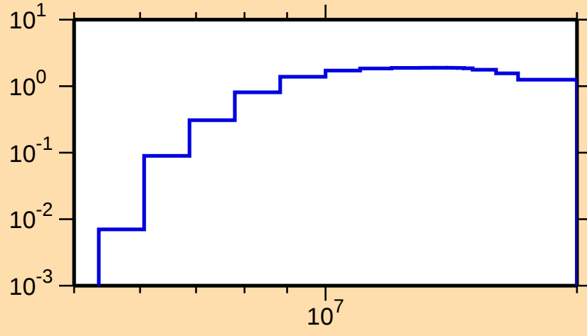
\sigma vs. E for ^{133}\text{Te}(n,2n)
