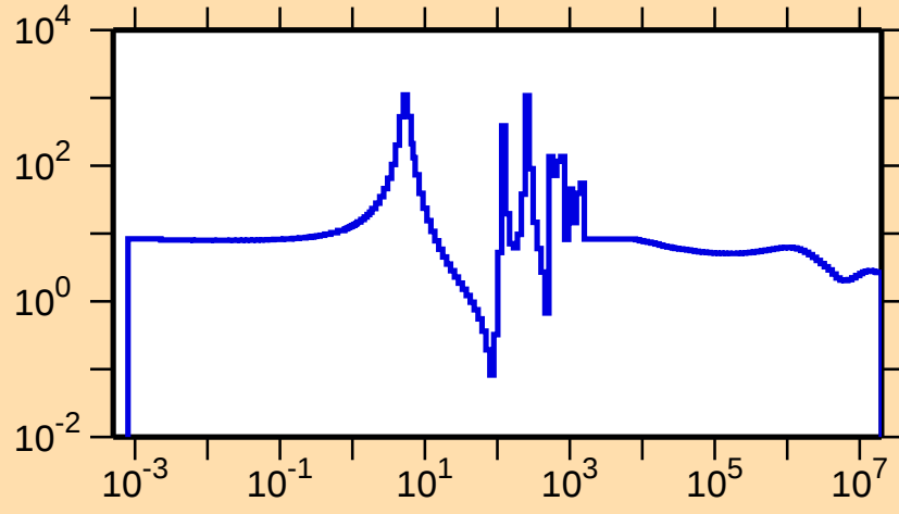
\sigma vs. E for ^{133}\text{Te}(n,\text{el.})
