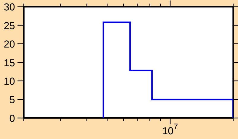
\Delta\sigma/\sigma vs. E for ^{133}\text{Te}(n,2n)
