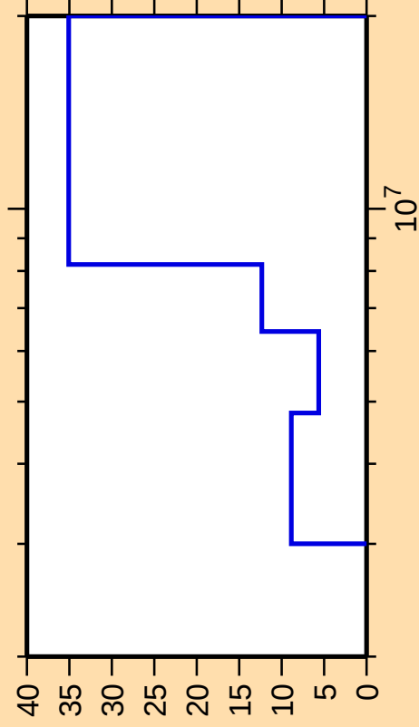
\Delta\sigma/\sigma vs. E for ^{133}\text{Te}(\text{n},\text{ncont.})
