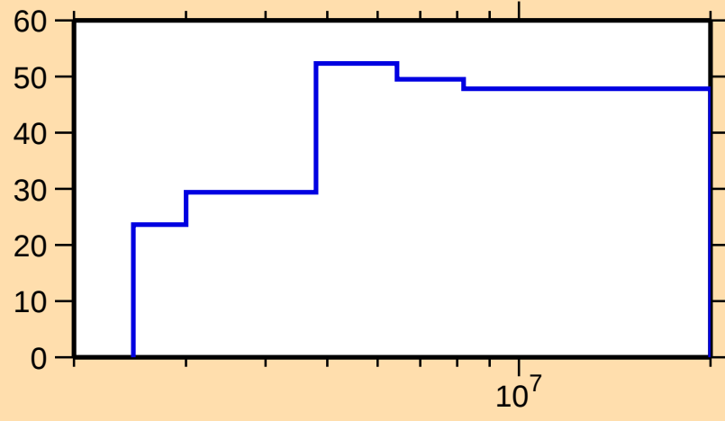
\Delta\sigma/\sigma vs. E for ^{133}\text{Te}(n,n_1)
