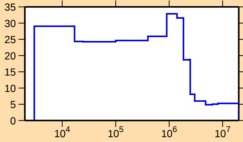
\Delta\sigma/\sigma vs. E for ^{133}\text{Te}(n,\text{nonel.})
