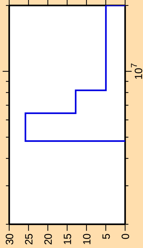
\Delta\sigma/\sigma vs. E for ^{133}\text{Te}(n,2n)
