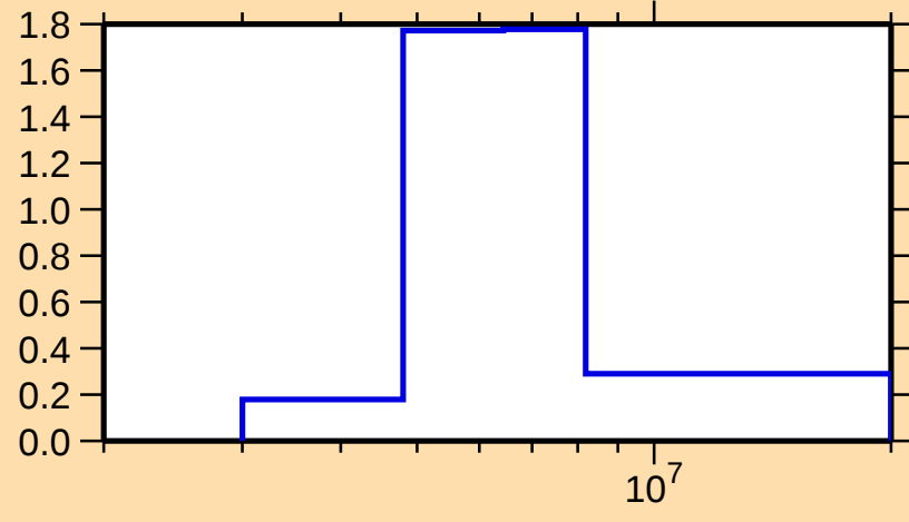
\sigma vs. E for ^{133}\text{Te}(n,n\text{cont.})
