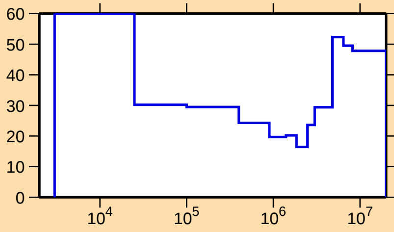
\Delta\sigma/\sigma vs. E for ^{133}\text{Te}(n,n_1)
