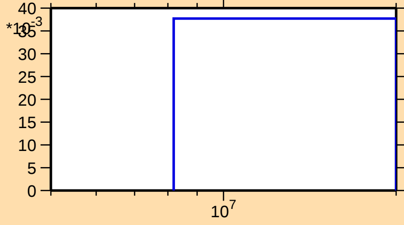
\sigma vs. E for ^{133}\text{Te}(n,3n)
