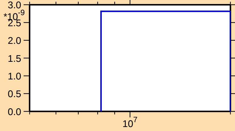
\sigma vs. E for ^{133}\text{Te}(\text{n},\text{nd})
