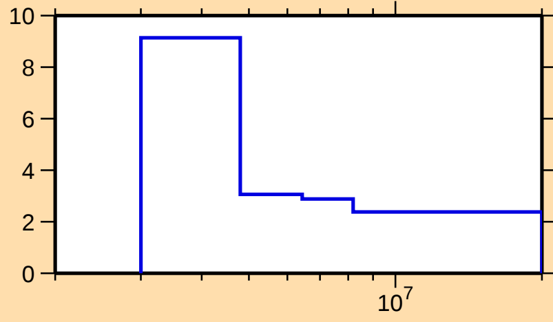
\Delta\sigma/\sigma vs. E for ^{133}\text{Te}(n,\text{tot.})
