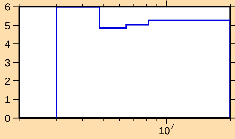
\Delta\sigma/\sigma vs. E for ^{133}\text{Te}(n,\text{nonel.})
