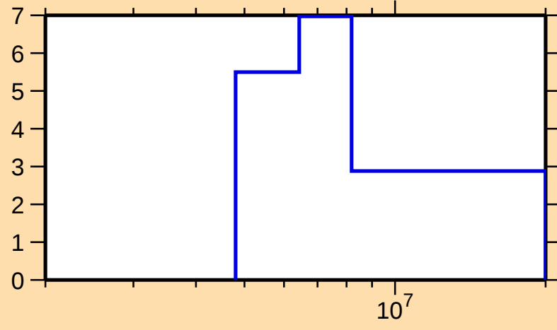
\Delta\sigma/\sigma vs. E for ^{133}\text{Te}(n,\text{el.})
