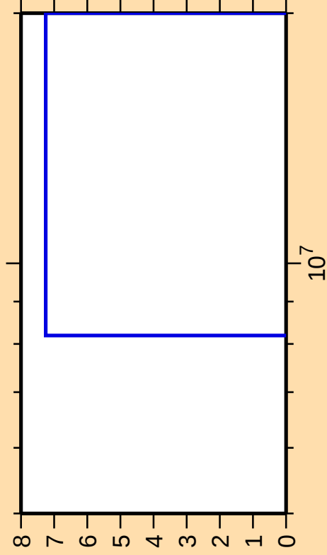
\Delta\sigma/\sigma vs. E for ^{133}\text{Te}(n,2np)
