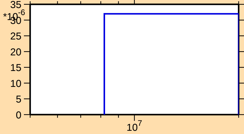
\sigma vs. E for ^{133}\text{Te}(n,np)
