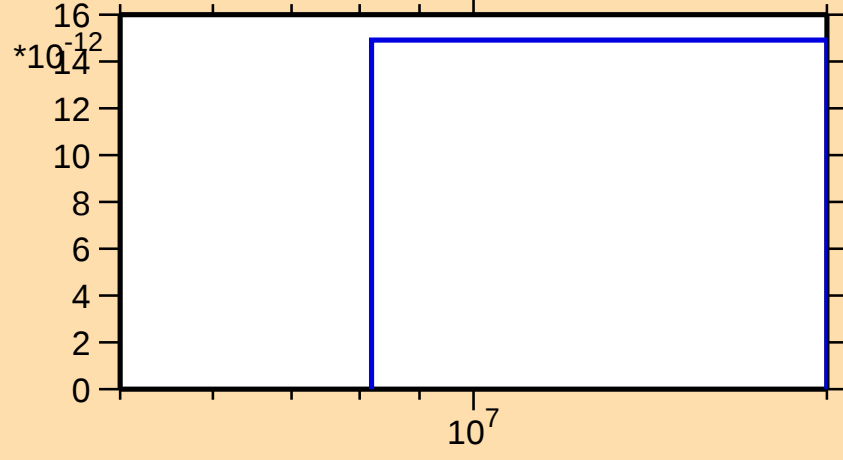
\sigma vs. E for ^{133}\text{Te}(n,nt)
