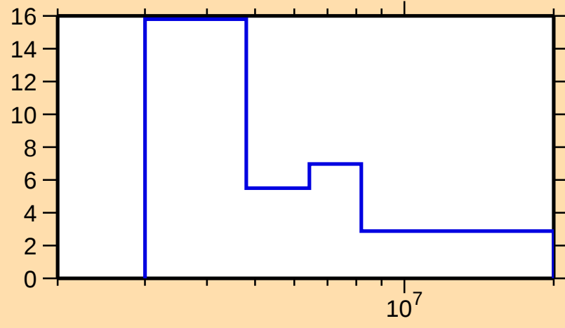
\Delta\sigma/\sigma vs. E for ^{133}\text{Te}(\text{n},\text{el.})
