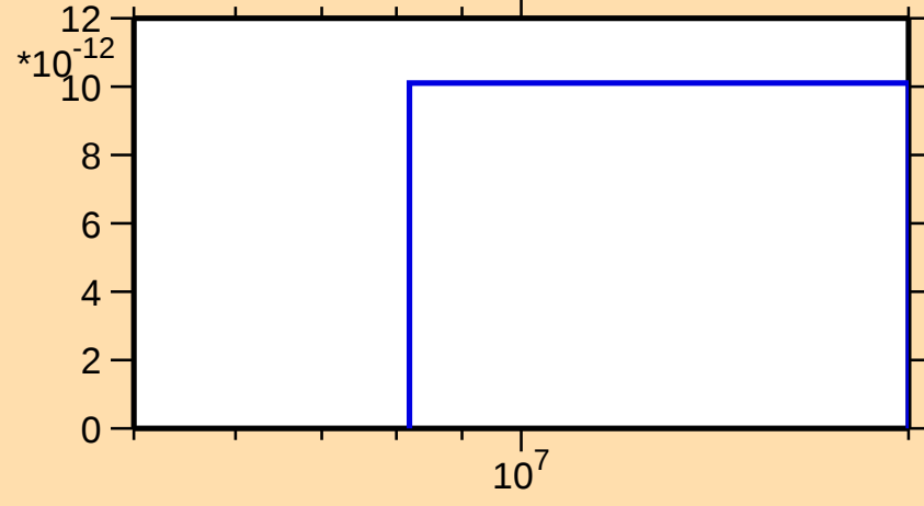
\sigma vs. E for ^{133}\text{Te}(n,2np)
