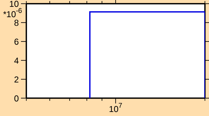
\sigma vs. E for ^{133}\text{Te}(n,t)
