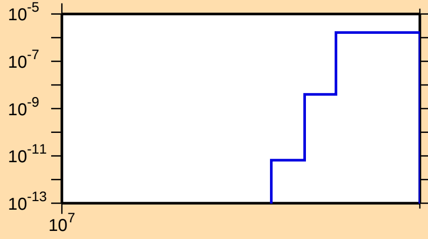
\sigma vs. E for ^{135}\text{Te}(n,nt)
