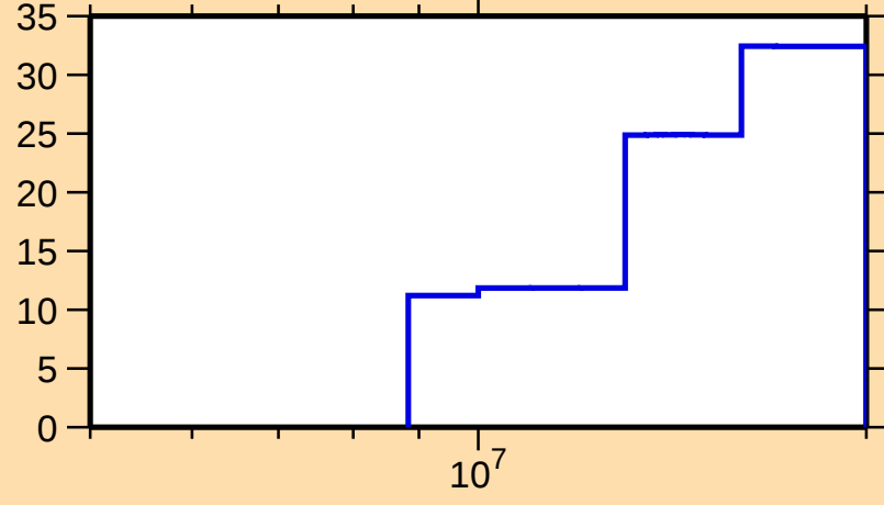
\Delta\sigma/\sigma vs. E for ^{135}\text{Te}(n,2n)
