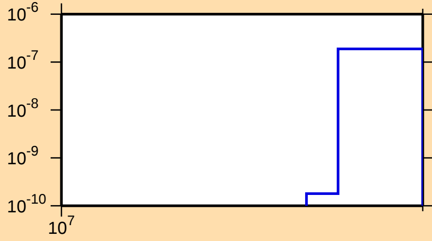
\sigma vs. E for ^{135}\text{Te}(n,2np)
