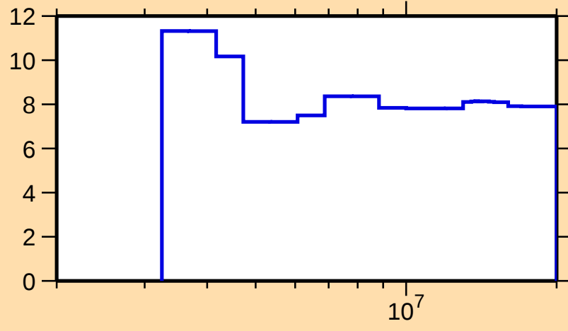
\Delta\sigma/\sigma vs. E for ^{135}\text{Te}(n,n\text{onel.})
