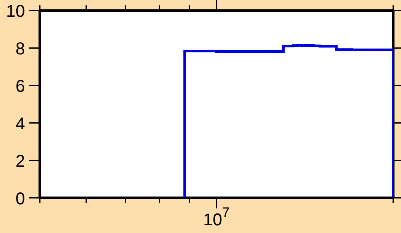
\Delta\sigma/\sigma vs. E for ^{135}\text{Te}(n,\text{nonel.})
