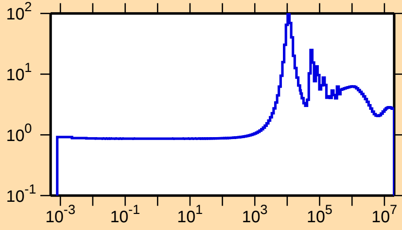
\sigma vs. E for ^{135}\text{Te}(n,\text{el.})
