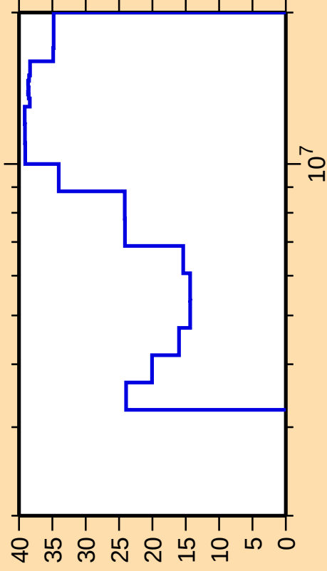
\Delta\sigma/\sigma vs. E for ^{135}\text{Te}(n,n\text{cont.})
