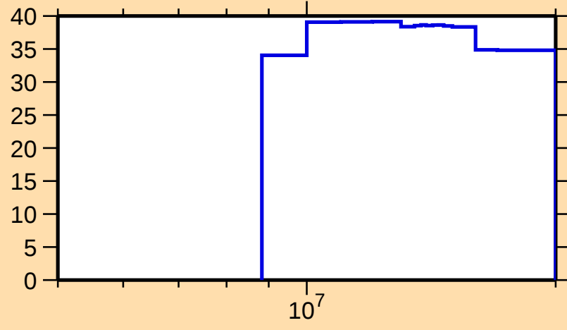
\Delta\sigma/\sigma vs. E for ^{135}\text{Te}(n,n\text{cont.})
