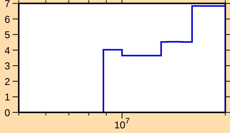
\Delta\sigma/\sigma vs. E for ^{135}\text{Te}(n,\text{tot.})
