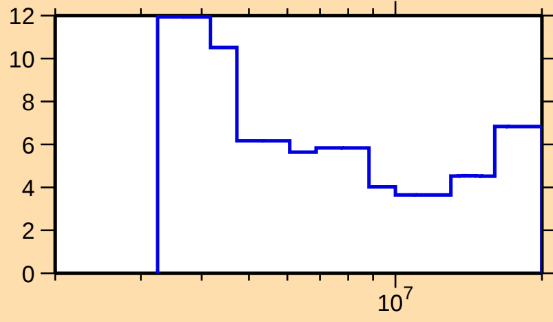
\Delta\sigma/\sigma vs. E for ^{135}\text{Te}(n,\text{tot.})
