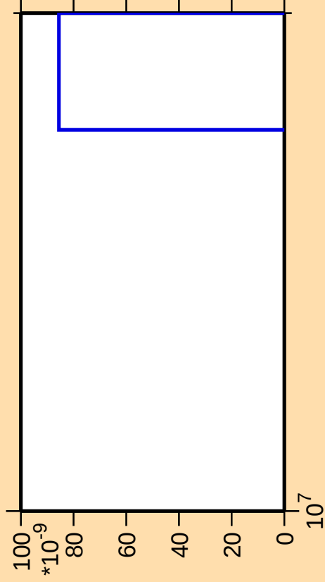
\Delta\sigma/\sigma vs. E for ^{135}\text{Te}(\text{mt } 11)
