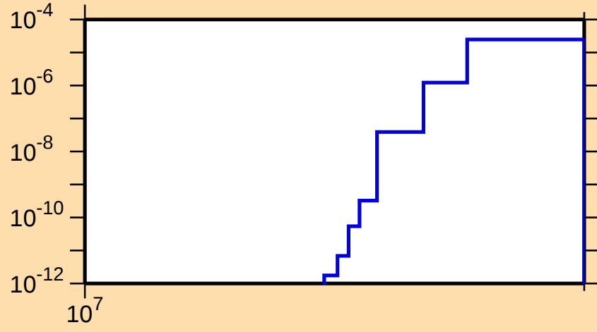
\sigma vs. E for ^{135}\text{Te}(n,\text{nd})
