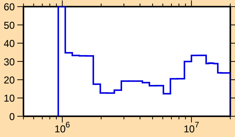
\Delta\sigma/\sigma vs. E for ^{135}\text{Te}(n,\text{inel.})
