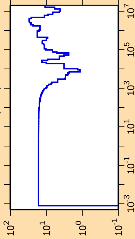
\Delta\sigma/\sigma vs. E for ^{135}\text{Te}(n,\text{el.})
