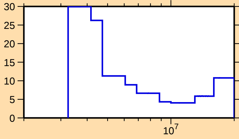
\Delta\sigma/\sigma vs. E for ^{135}\text{Te}(n,\text{el.})
