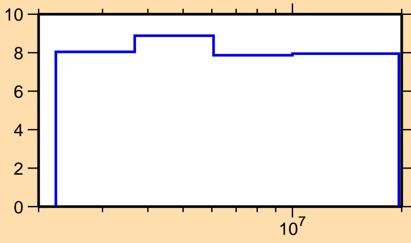
\Delta\sigma/\sigma vs. E for ^{135}\text{Te}(n,\text{nonel.})
