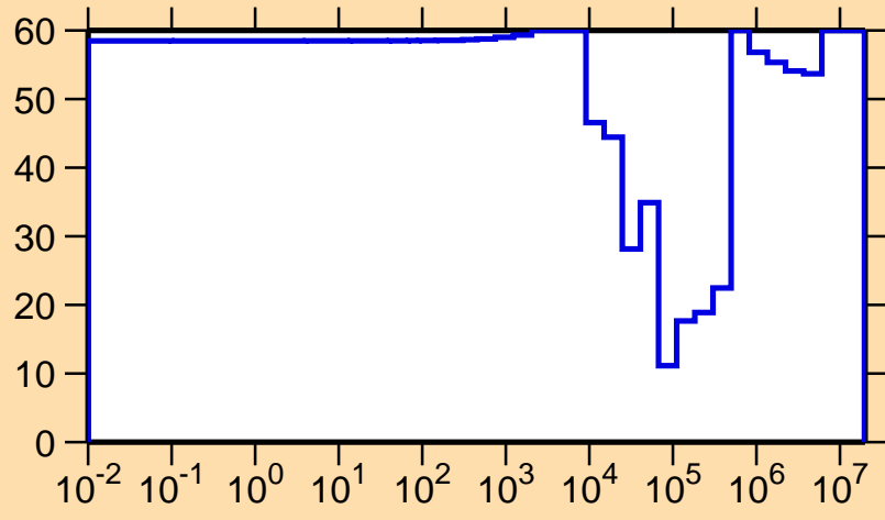
\Delta\sigma/\sigma vs. E for ^{135}\text{Te}(n,\gamma)
