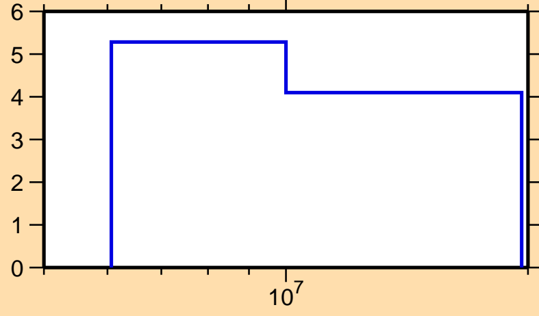
\Delta\sigma/\sigma vs. E for ^{135}\text{Te}(n,\text{tot.})
