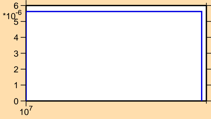
\sigma vs. E for ^{135}\text{Te}(n,np)
