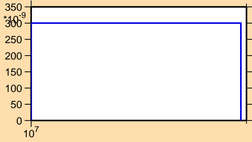
\sigma vs. E for ^{135}\text{Te}(n,\text{nd})
