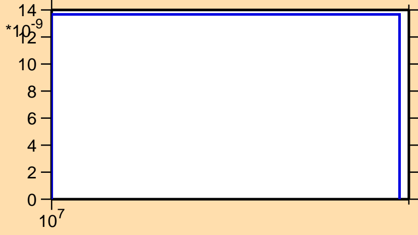
\sigma vs. E for ^{135}\text{Te}(n,nt)
