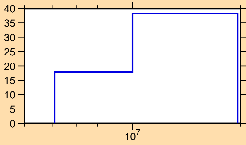
\Delta\sigma/\sigma vs. E for ^{135}\text{Te}(n,n\text{cont.})
