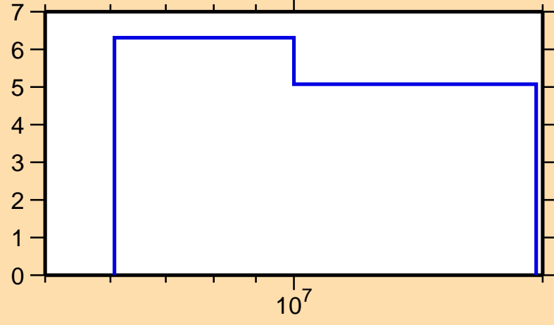
\Delta\sigma/\sigma vs. E for ^{135}\text{Te}(n,\text{el.})
