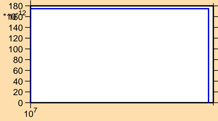
\sigma vs. E for ^{135}\text{Te}(n,2n\alpha)
