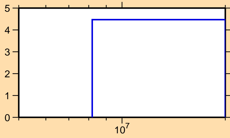
\Delta\sigma/\sigma vs. E for ^{135}\text{Te}(n,el.)
