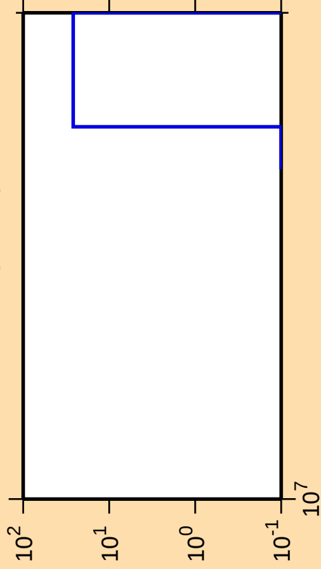
\Delta\sigma/\sigma vs. E for ^{137}\text{Te}(n,3n\alpha)
