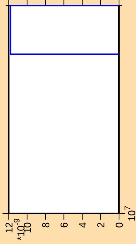
\Delta\sigma/\sigma vs. E for ^{137}\text{Te}(\text{mt } 42)
