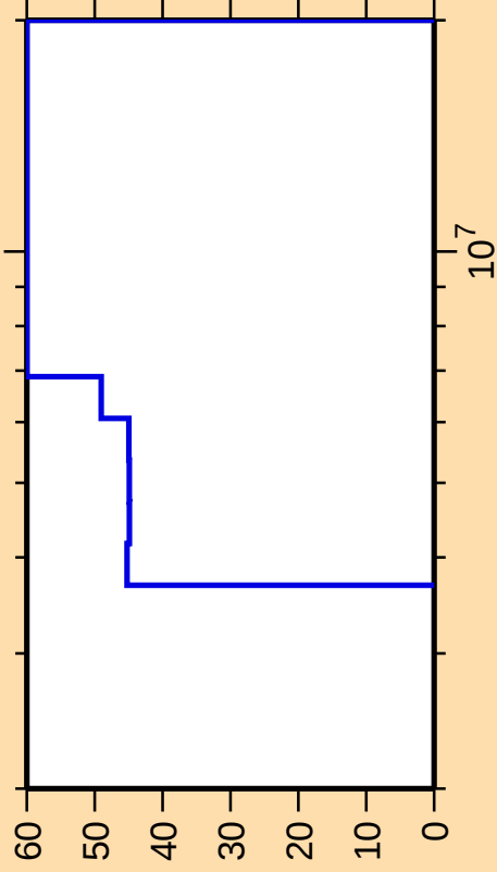
\Delta\sigma/\sigma vs. E for ^{137}\text{Te}(n,n\text{cont.})
