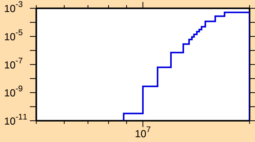
\sigma vs. E for ^{137}\text{Te}(n,t)
