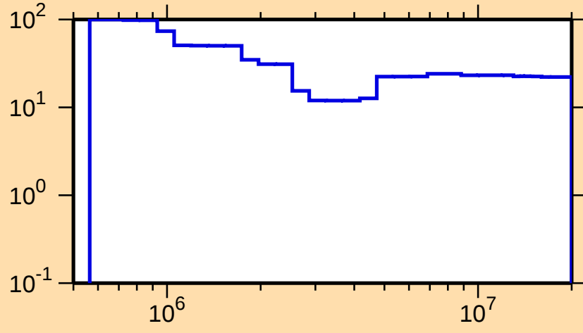
\Delta\sigma/\sigma vs. E for ^{137}\text{Te}(n,\text{inel.})
