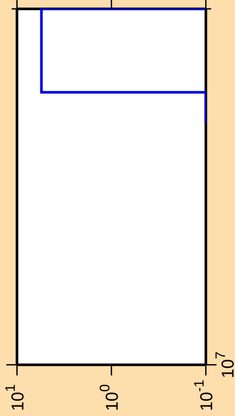
\Delta\sigma/\sigma vs. E for ^{137}\text{Te}(\text{mt } 11)
