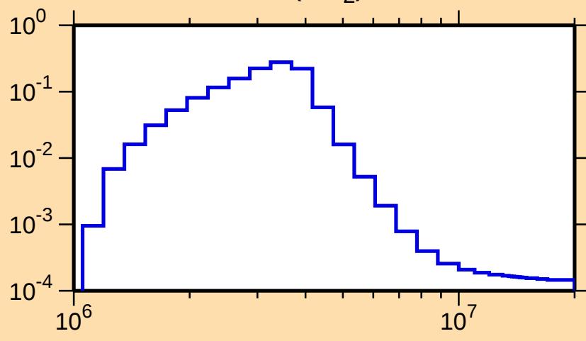
\sigma vs. E for ^{137}\text{Te}(n,n_2)
