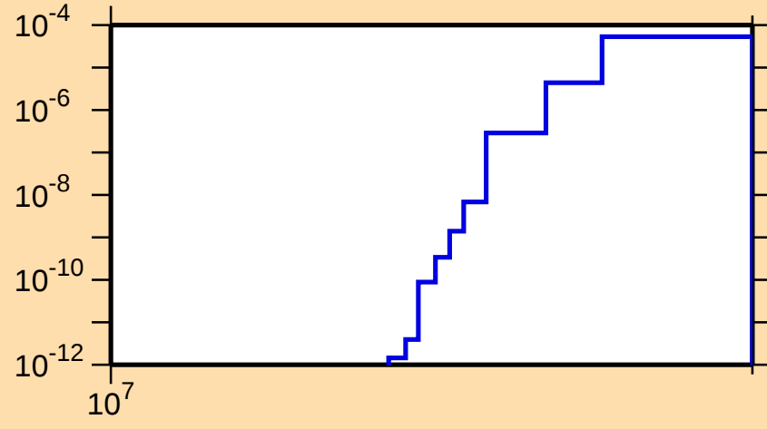
\sigma vs. E for ^{137}\text{Te}(n,np)
