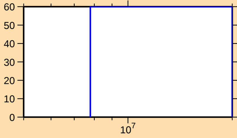
\Delta\sigma/\sigma vs. E for ^{137}\text{Te}(n,n\text{cont.})
