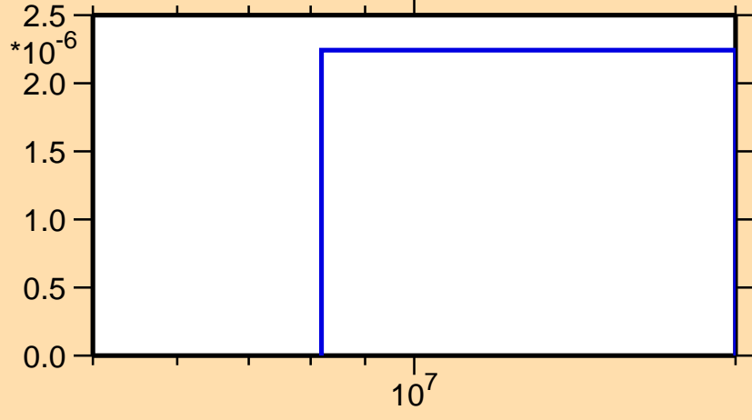
\sigma vs. E for ^{137}\text{Te}(n,nt)
