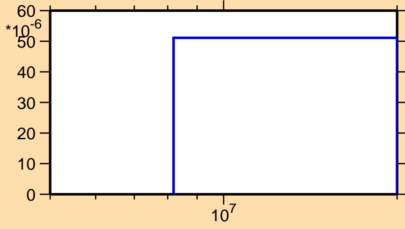
\sigma vs. E for ^{137}\text{Te}(n,p)
