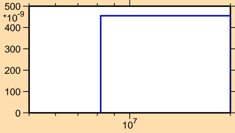
\sigma vs. E for ^{137}\text{Te}(n,2n\alpha)
