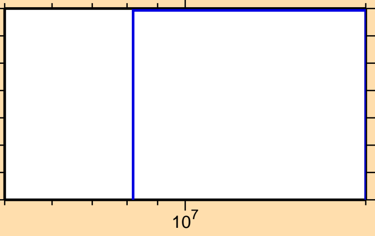
\sigma vs. E for ^{137}\text{Te}(n,d)
