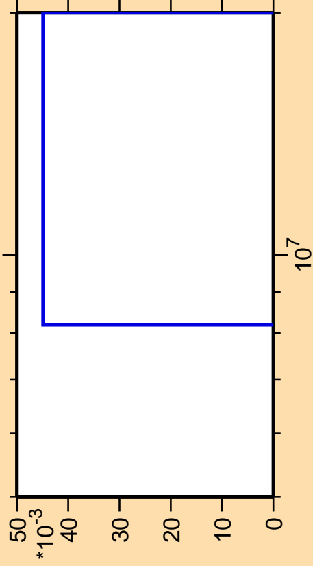
\Delta\sigma/\sigma vs. E for ^{137}\text{Te}(\text{mt } 11)
