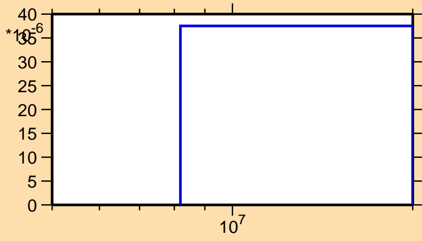
\sigma vs. E for ^{137}\text{Te}(n,t)
