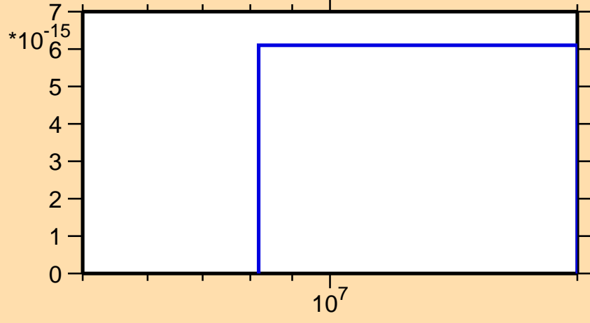
\sigma vs. E for ^{137}\text{Te}(\text{mt } 11)
