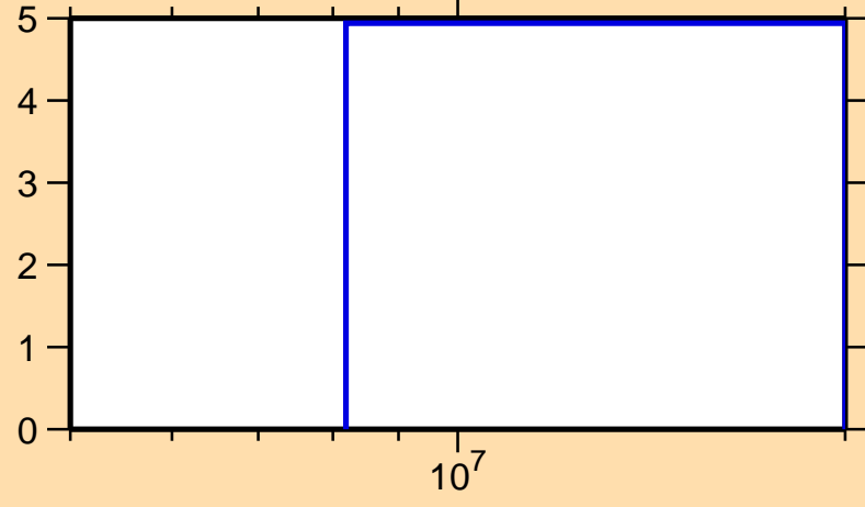
\Delta\sigma/\sigma vs. E for ^{137}\text{Te}(n,el.)
