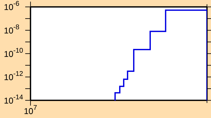
\sigma vs. E for ^{228}\text{Th}(n,\text{nt})
