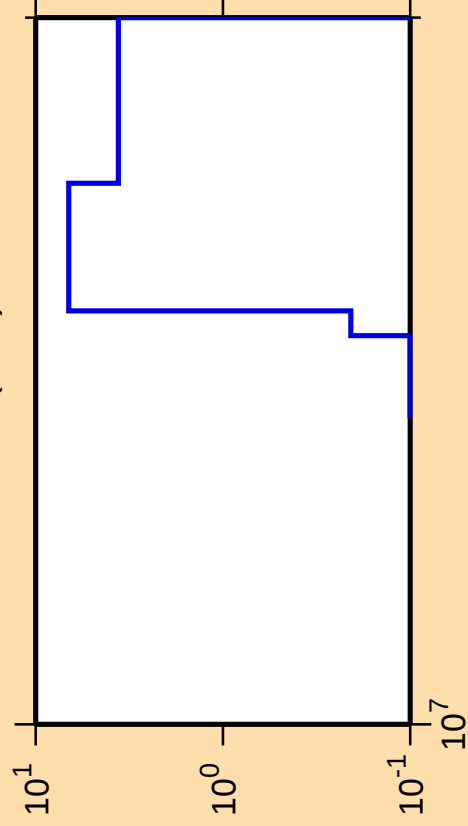
\Delta\sigma/\sigma vs. E for ^{228}\text{Th}(n,\text{nt})
