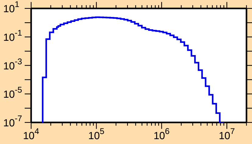
\sigma vs. E for ^{233}\text{Th}(n,n_3)
