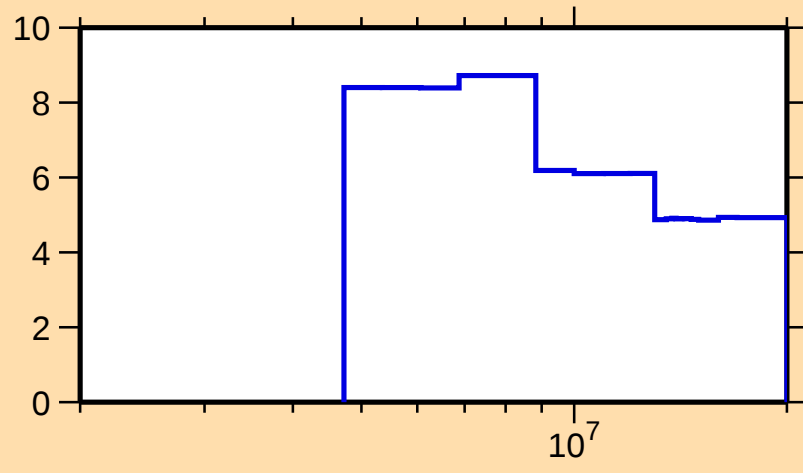
\Delta\sigma/\sigma vs. E for ^{233}\text{Th}(n,\text{tot.})
