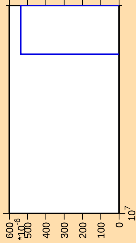
\Delta\sigma/\sigma vs. E for ^{233}\text{Th}(\text{mt } 42)
