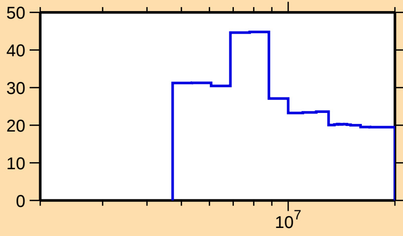
\Delta\sigma/\sigma vs. E for ^{233}\text{Th}(n,\text{inel.})
