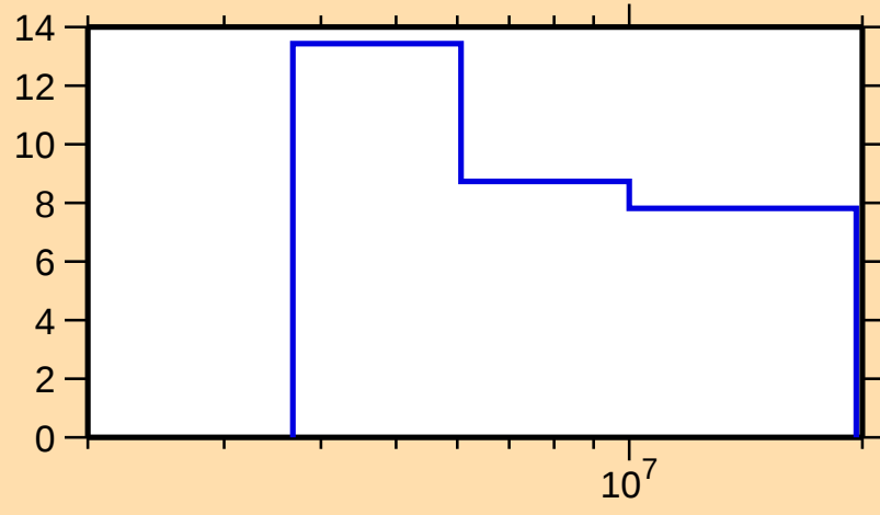
\Delta\sigma/\sigma vs. E for ^{233}\text{Th}(n,\text{nonel.})
