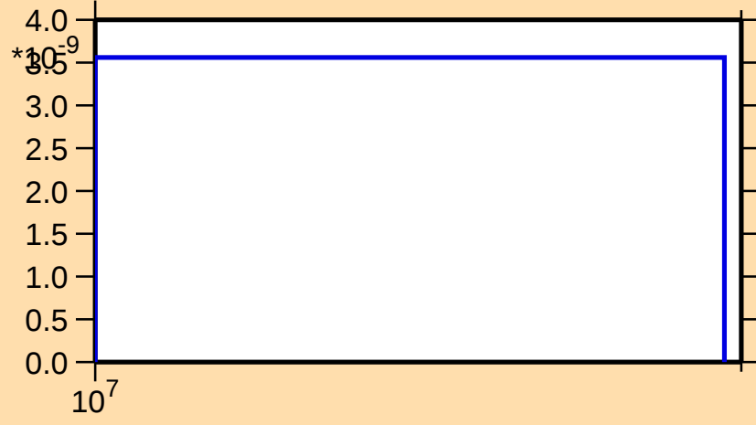
\sigma vs. E for ^{233}\text{Th}(n,nt)
