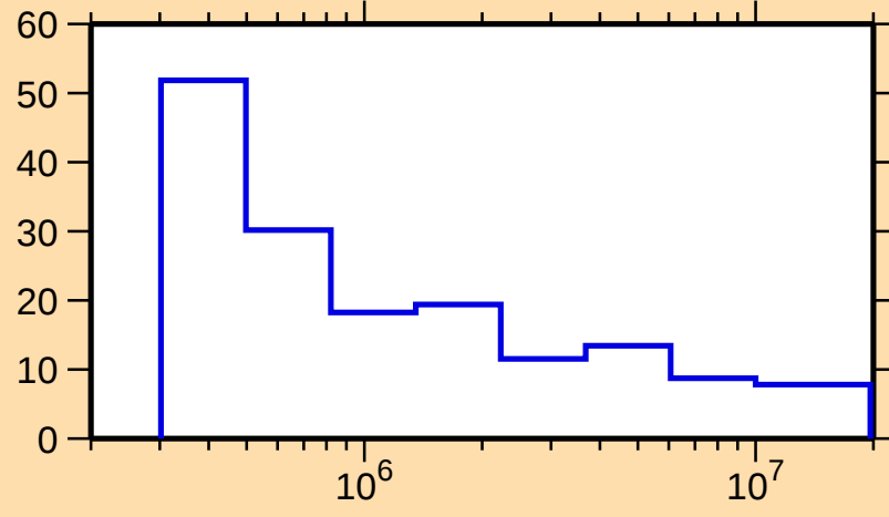
\Delta\sigma/\sigma vs. E for ^{233}\text{Th}(n,\text{nonel.})
