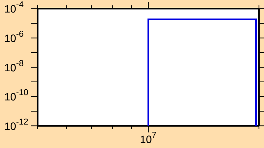
\sigma vs. E for ^{233}\text{Th}(n,t)
