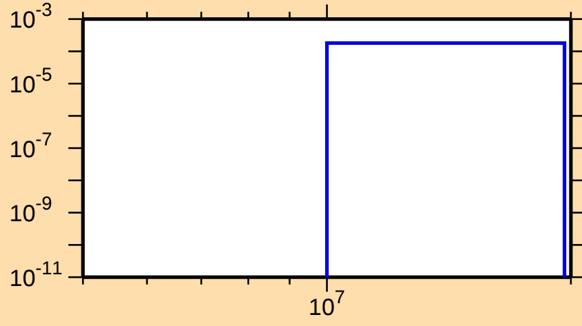
\sigma vs. E for ^{233}\text{Th}(n,np)
