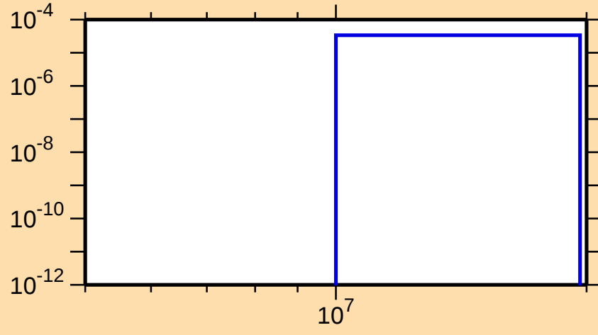
\sigma vs. E for ^{233}\text{Th}(n,d)
