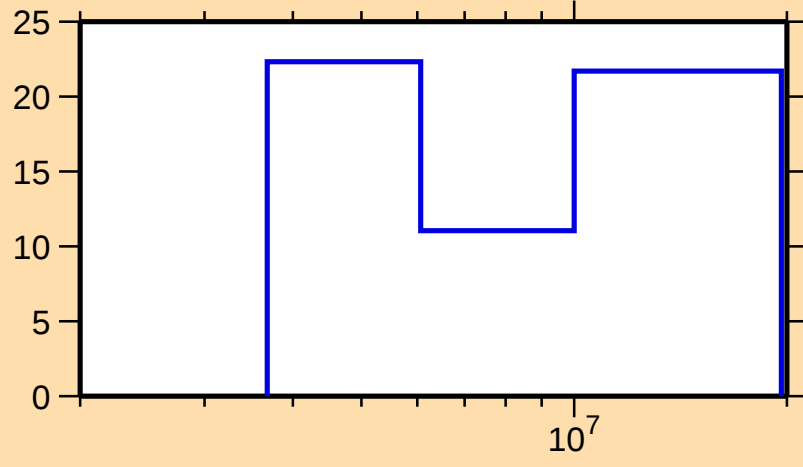
\Delta\sigma/\sigma vs. E for ^{233}\text{Th}(n,2n)
