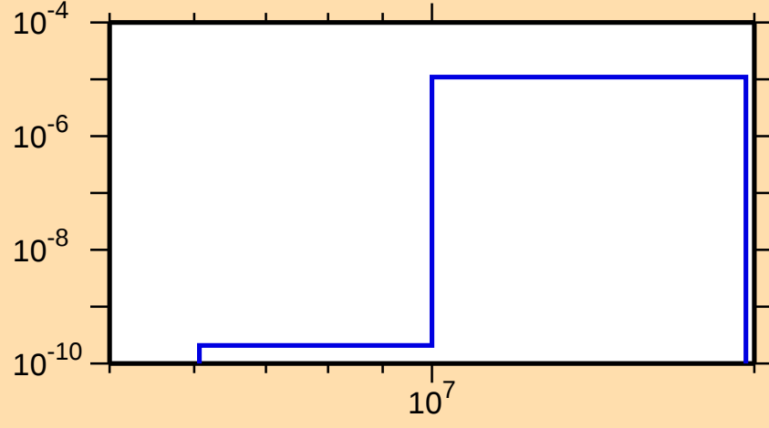
\sigma vs. E for ^{233}\text{Th}(n,n\alpha)
