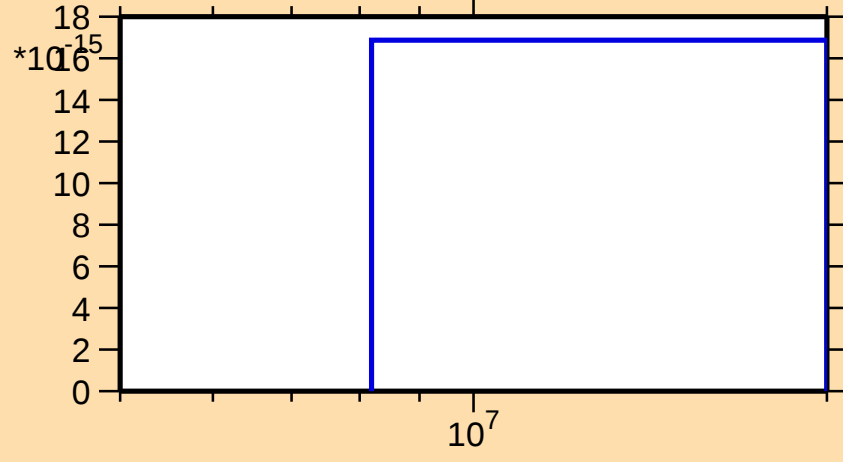
\sigma vs. E for ^{233}\text{Th}(n,\text{He3})
