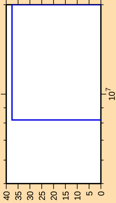
\Delta\sigma/\sigma vs. E for ^{233}\text{Th}(n,d)
