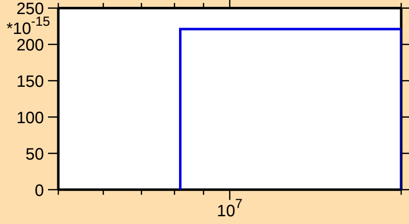
\sigma vs. E for ^{233}\text{Th}(n,3n\alpha)
