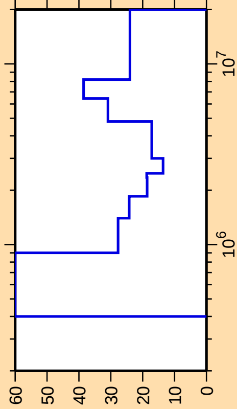
\Delta\sigma/\sigma vs. E for ^{233}\text{Th}(n,\text{ncont.})
