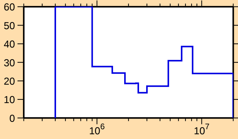
\Delta\sigma/\sigma vs. E for ^{233}\text{Th}(n,n\text{cont.})
