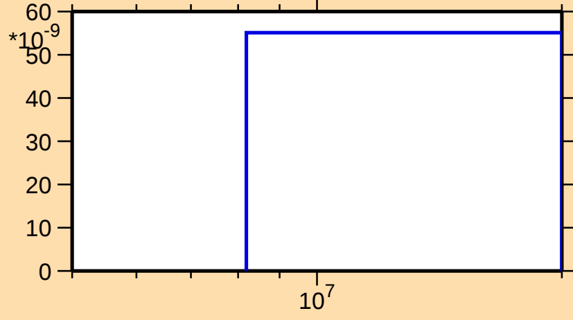
\sigma vs. E for ^{233}\text{Th}(n,2n\alpha)
