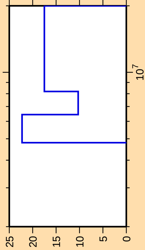
\Delta\sigma/\sigma vs. E for ^{233}\text{Th}(n,2n)
