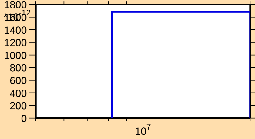
\sigma vs. E for ^{233}\text{Th}(n,2np)
