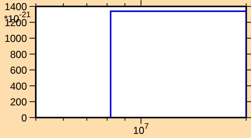
\sigma vs. E for ^{233}\text{Th}(\text{mt } 42)
