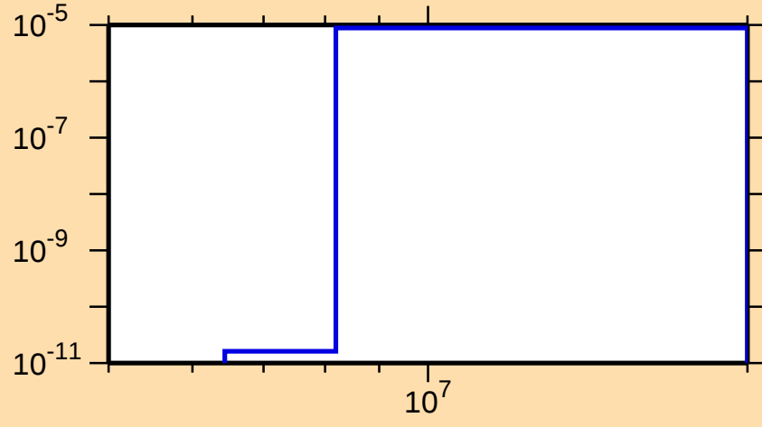
\sigma vs. E for ^{233}\text{Th}(n,n\alpha)
