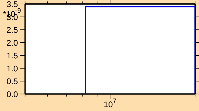
\sigma vs. E for ^{233}\text{Th}(n,nt)
