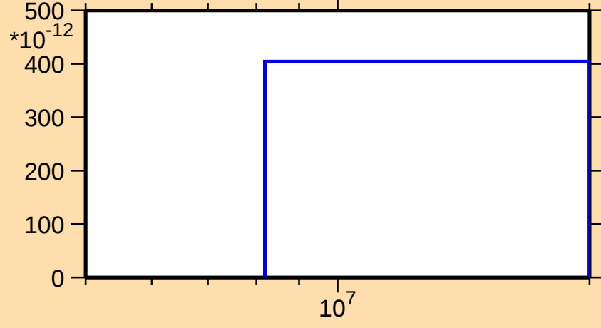
\sigma vs. E for ^{233}\text{Th}(n,\text{nd})
