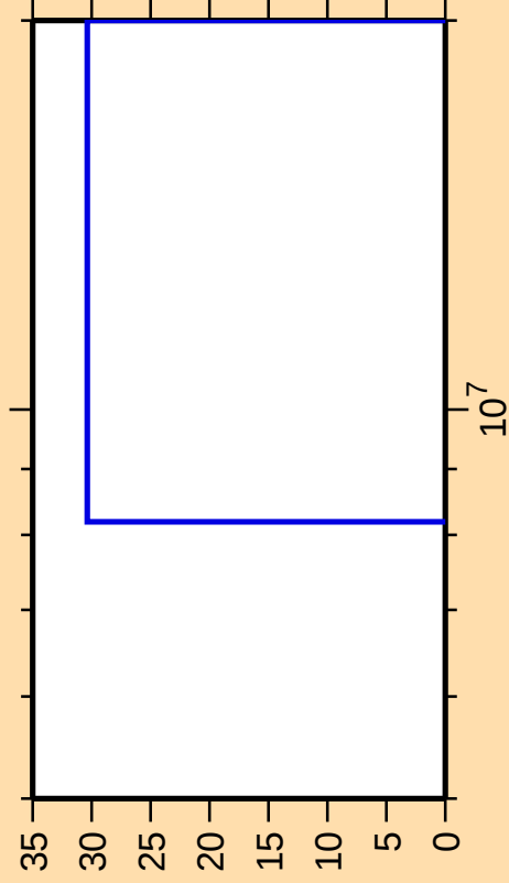
\Delta\sigma/\sigma vs. E for ^{233}\text{Th}(n,t)
