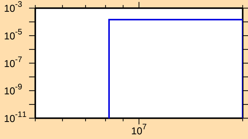
\sigma vs. E for ^{233}\text{Th}(n,np)
