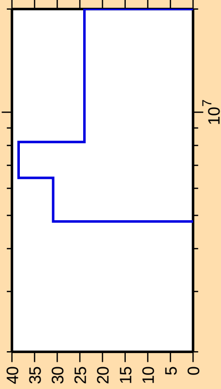
\Delta\sigma/\sigma vs. E for ^{233}\text{Th}(n,n\text{cont.})
