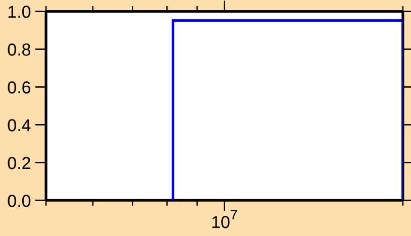
\sigma vs. E for ^{233}\text{Th}(n,3n)
