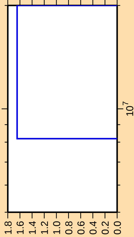
\Delta\sigma/\sigma vs. E for ^{233}\text{Th}(n,3n\alpha)
