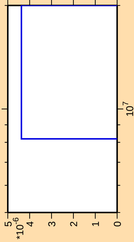
\Delta\sigma/\sigma vs. E for ^{233}\text{Th}(\text{mt } 42)
