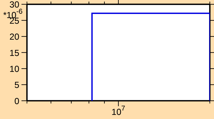
\sigma vs. E for ^{233}\text{Th}(n,d)
