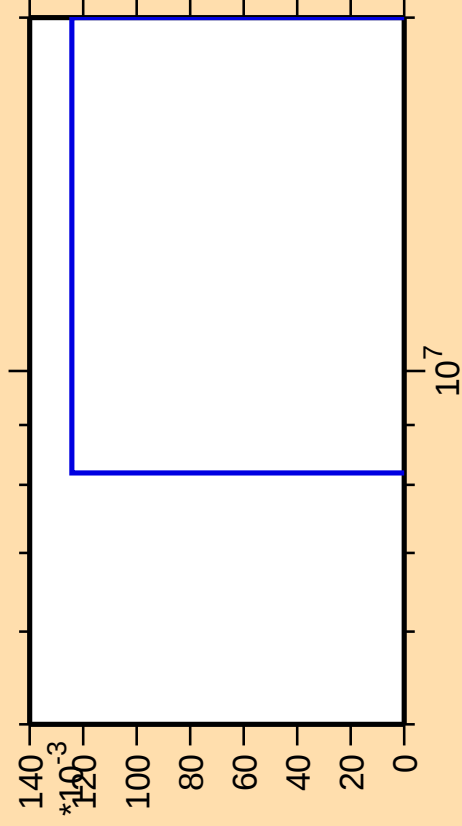
\Delta\sigma/\sigma vs. E for ^{233}\text{Th}(n,\text{He3})
