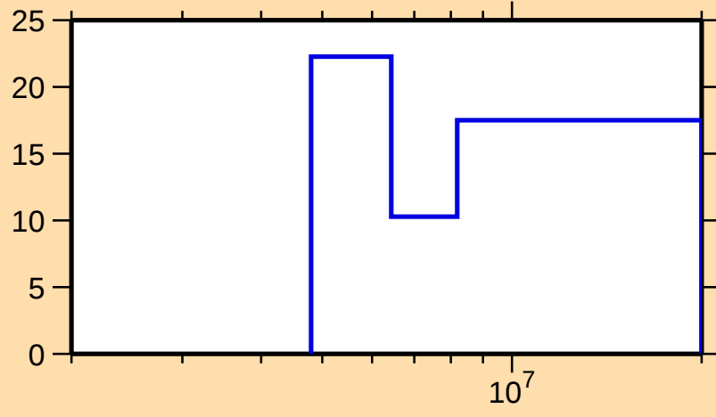
\Delta\sigma/\sigma vs. E for ^{233}\text{Th}(n,2n)
