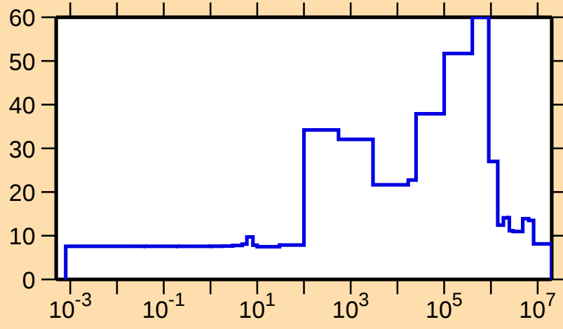
\Delta\sigma/\sigma vs. E for ^{233}\text{Th}(n,\text{el.})
