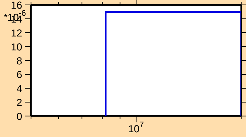
\sigma vs. E for ^{233}\text{Th}(n,t)
