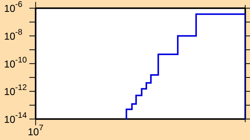
\sigma vs. E for ^{151}\text{Tm}(n,\text{pt})
