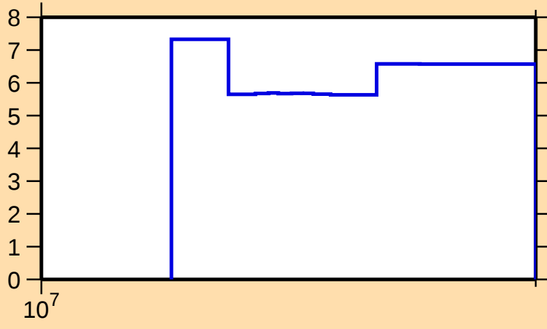
\Delta\sigma/\sigma vs. E for ^{151}\text{Tm}(n,\text{el.})
