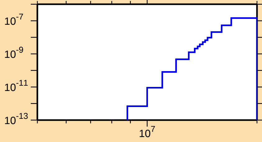
\sigma vs. E for ^{151}\text{Tm}(\text{mt117})
