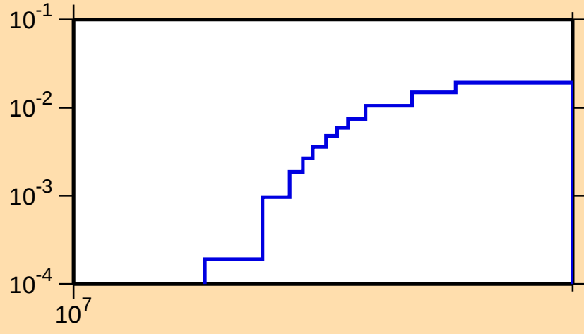
\sigma vs. E for ^{151}\text{Tm}(n,2n)
