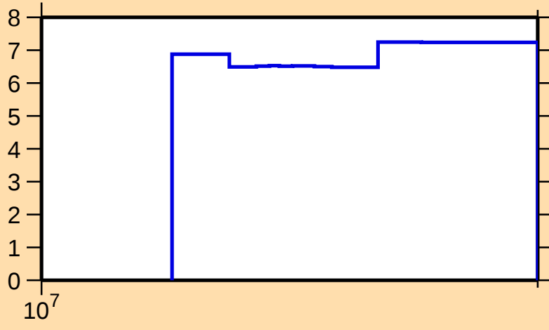
\Delta\sigma/\sigma vs. E for ^{151}\text{Tm}(n,\text{nonel.})
