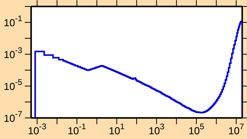
\sigma vs. E for ^{151}\text{Tm}(n,p\alpha)
