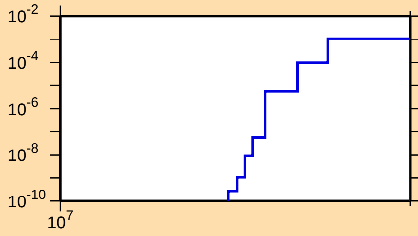
\sigma vs. E for ^{151}\text{Tm}(n,2np)
