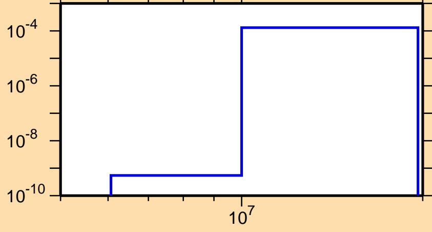
\sigma vs. E for ^{151}\text{Tm}(n,\text{pd})
