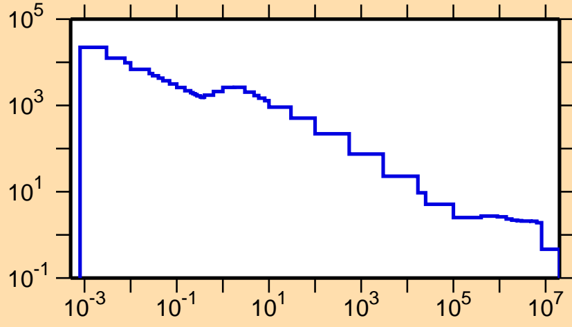
\sigma vs. E for ^{151}\text{Tm}(n,p)
