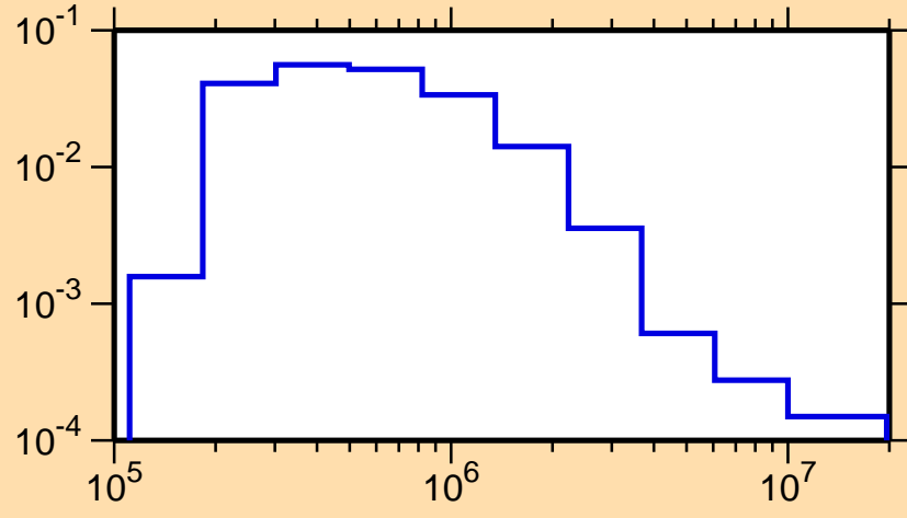
\sigma vs. E for ^{159}\text{Tm}(n,n_4)
