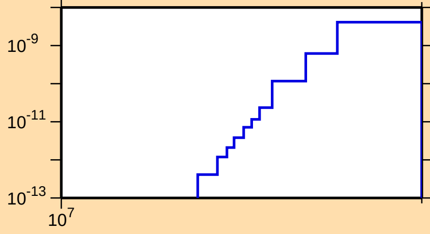
\sigma vs. E for ^{162}\text{Tm} (mt 45)
