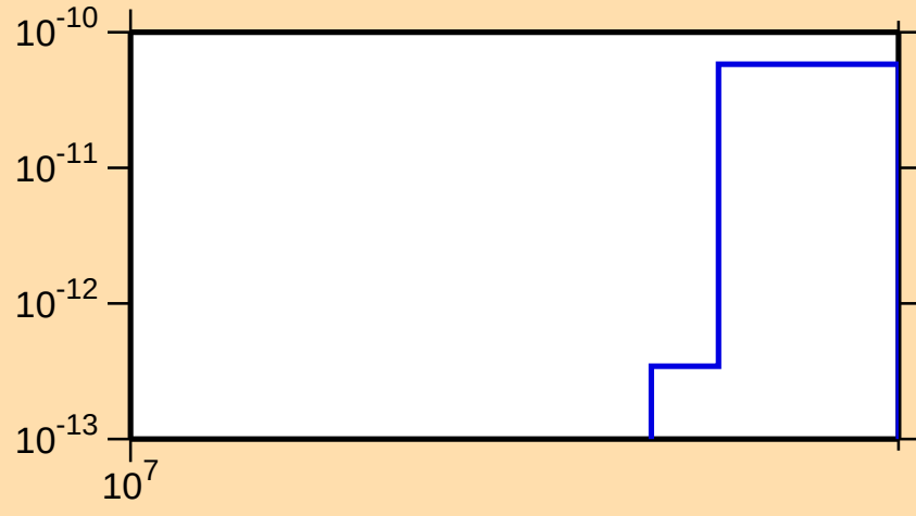
\sigma vs. E for ^{162}\text{Tm} (mt 34)
