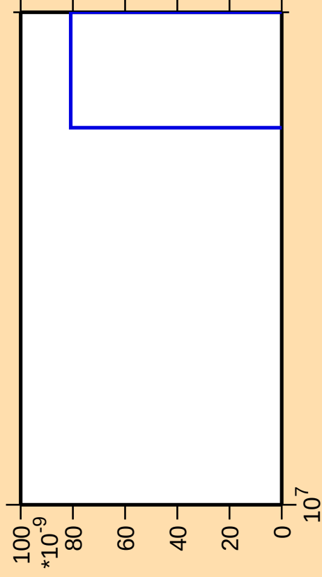
\Delta\sigma/\sigma vs. E for ^{162}\text{Tm}(\text{mt } 11)
