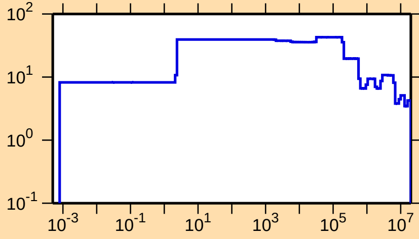
\Delta\sigma/\sigma vs. E for ^{162}\text{Tm}(n,\text{el.})
