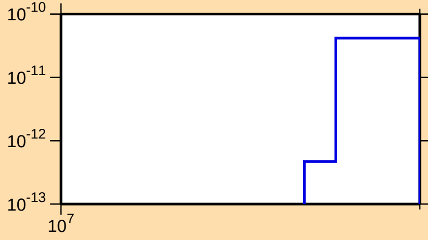
\sigma vs. E for ^{162}\text{Tm}(n,\text{pt})
