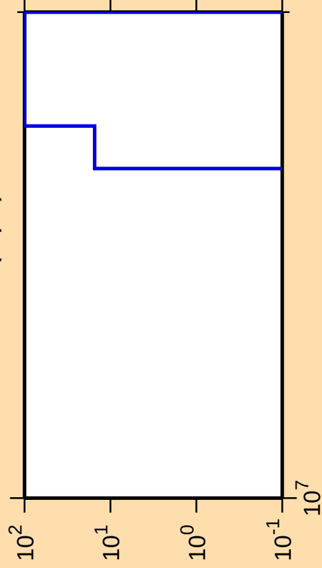
\Delta\sigma/\sigma vs. E for ^{162}\text{Tm}(n,\text{pd})
