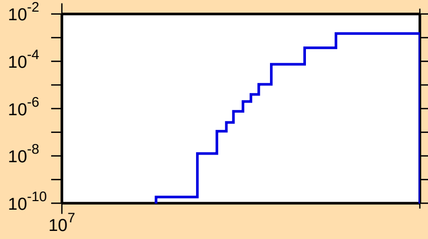
\sigma vs. E for ^{162}\text{Tm}(n,2np)
