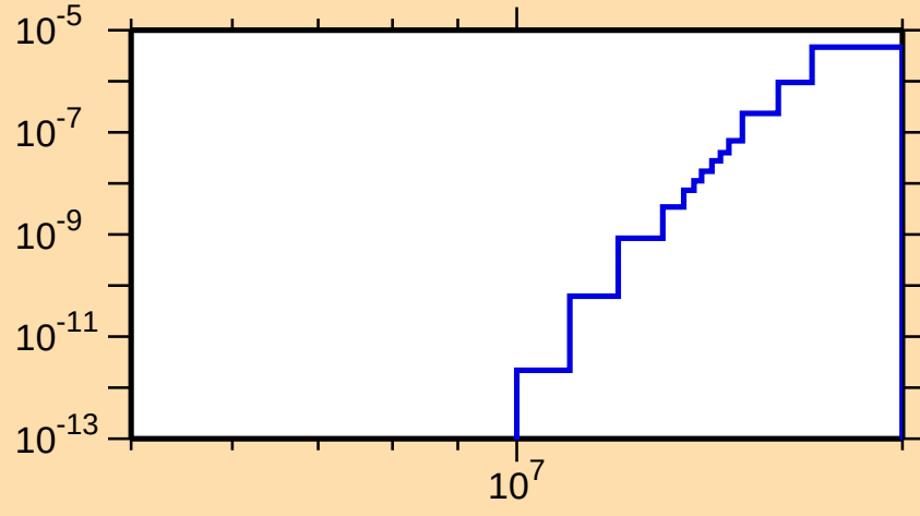
\sigma vs. E for ^{162}\text{Tm}(n,\text{He}3)
