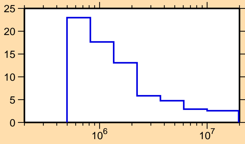
\Delta\sigma/\sigma vs. E for ^{162}\text{Tm}(n, nonel.)
