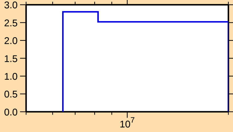
\Delta\sigma/\sigma vs. E for ^{162}\text{Tm}(n,\text{nonel.})
