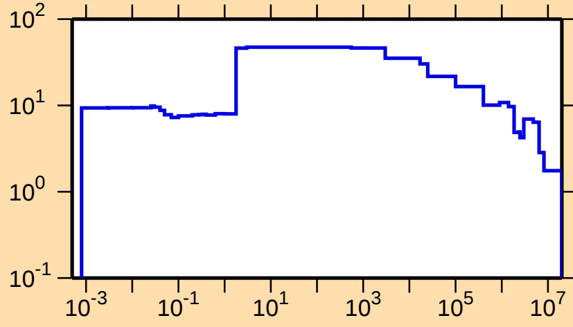
\Delta\sigma/\sigma vs. E for ^{162}\text{Tm}(n,\text{tot.})
