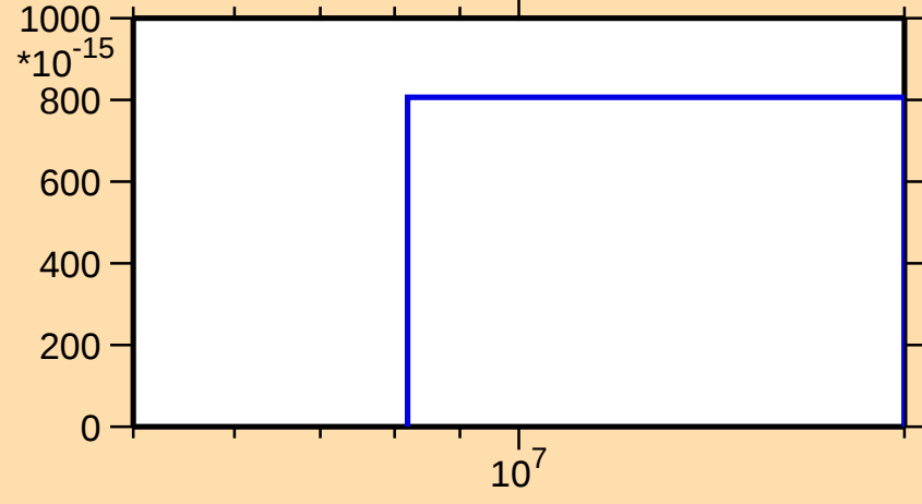
\sigma vs. E for ^{162}\text{Tm}(n,\text{pd})
