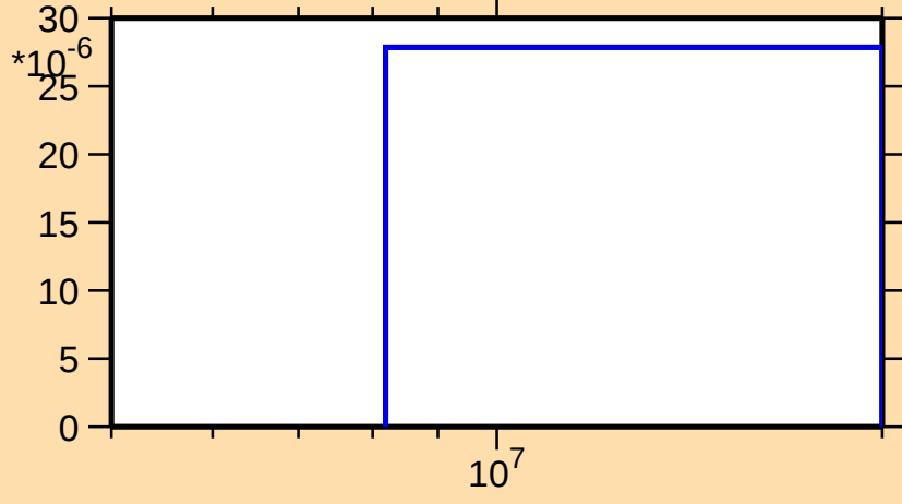
\sigma vs. E for ^{162}\text{Tm}(n,3n)
