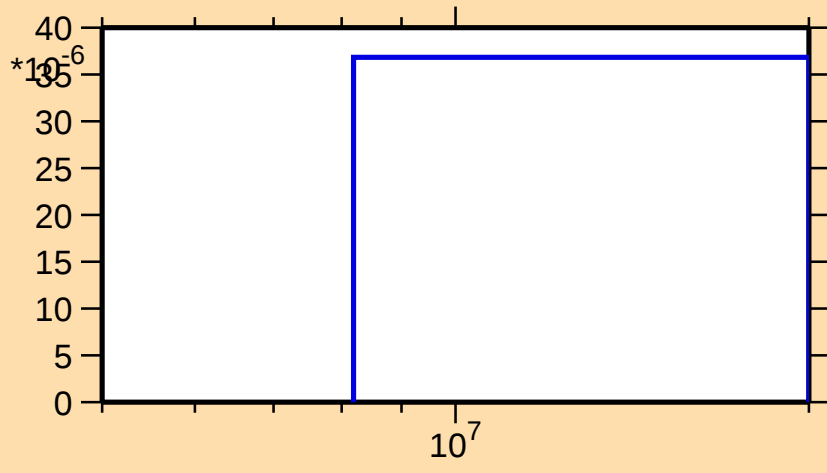
\sigma vs. E for ^{162}\text{Tm}(n,2np)
