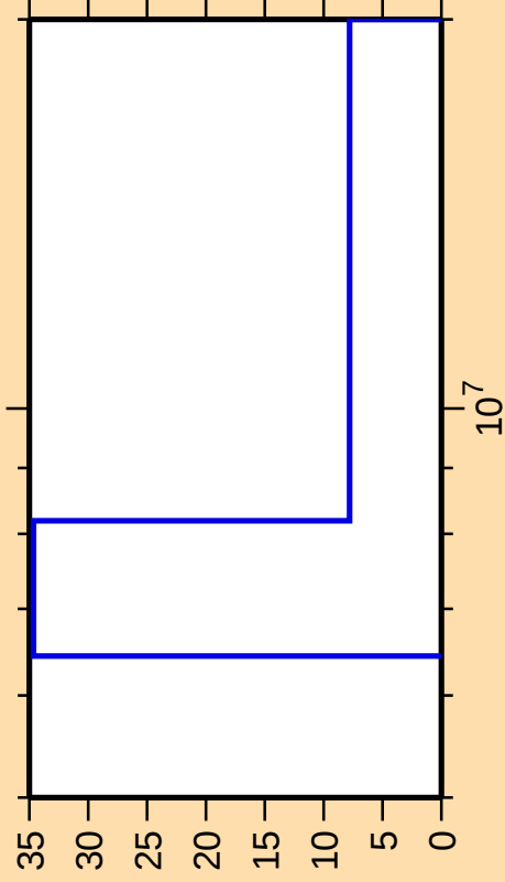
\Delta\sigma/\sigma vs. E for ^{162}\text{Tm}(n,2n)
