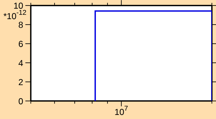
\sigma vs. E for ^{162}\text{Tm}(\text{mt117})
