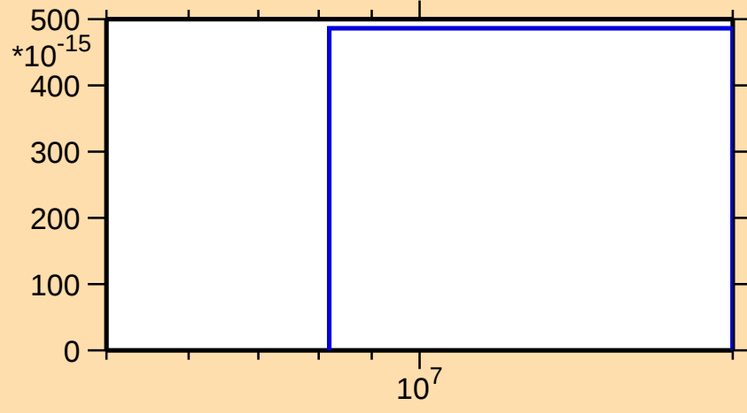
\sigma vs. E for ^{162}\text{Tm} (mt 34)
