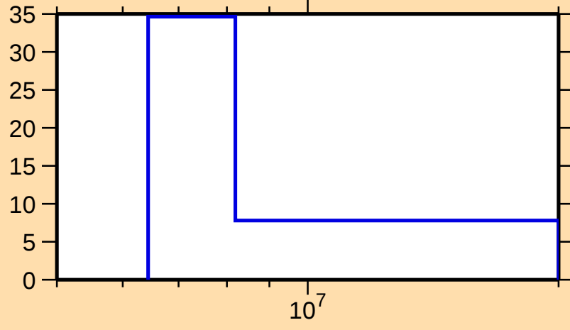
\Delta\sigma/\sigma vs. E for ^{162}\text{Tm}(n,2n)
