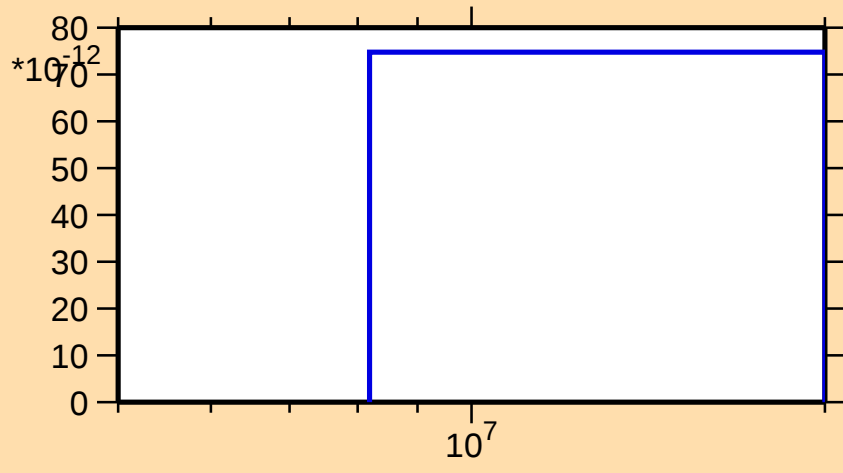
\sigma vs. E for ^{162}\text{Tm} (mt 45)
