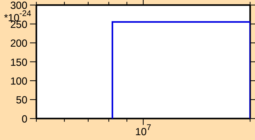
\sigma vs. E for ^{162}\text{Tm} (mt 11)
