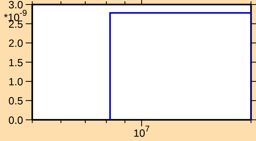
\sigma vs. E for ^{162}\text{Tm}(n,nt)
