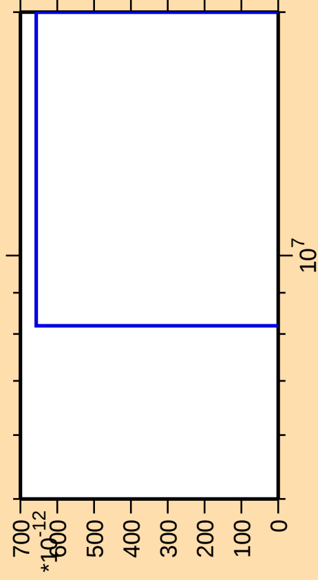
\Delta\sigma/\sigma vs. E for ^{162}\text{Tm} (mt 11)
