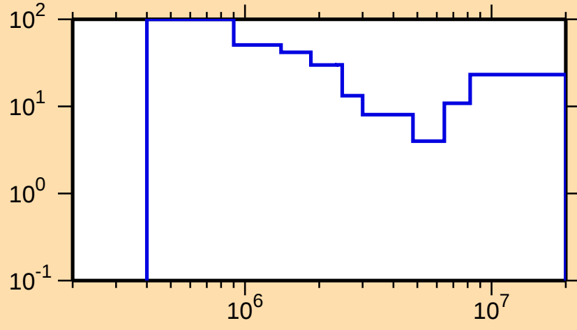
\Delta\sigma/\sigma vs. E for ^{162}\text{Tm}(n,n\text{cont.})
