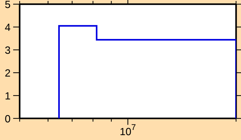
\Delta\sigma/\sigma vs. E for ^{162}\text{Tm}(n,\text{el.})
