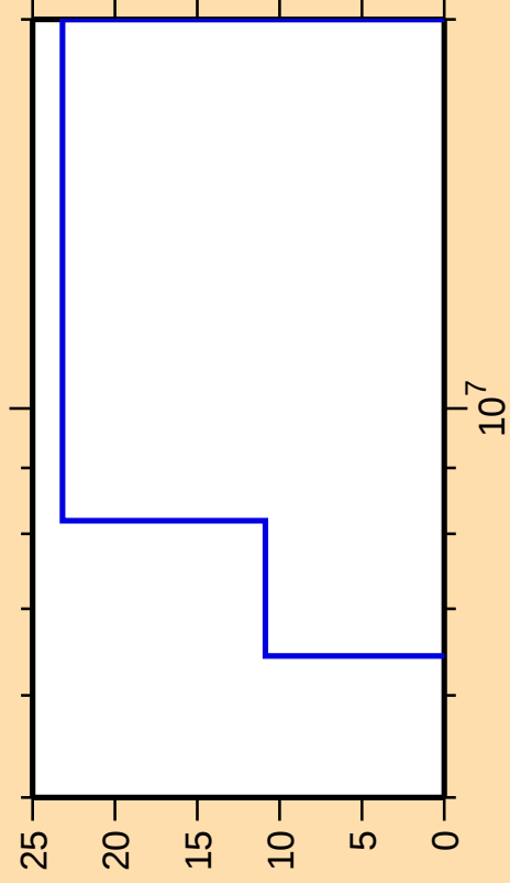
\Delta\sigma/\sigma vs. E for ^{162}\text{Tm}(n,n\text{cont.})
