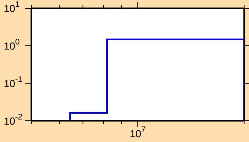
\sigma vs. E for ^{162}\text{Tm}(n,2n)
