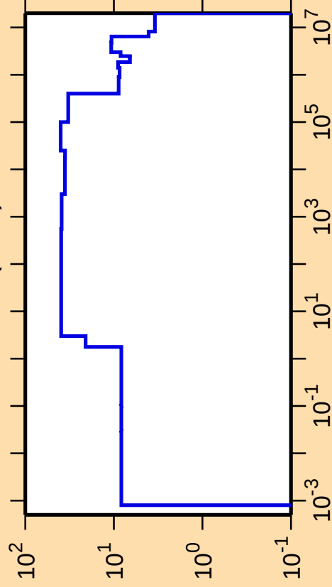
\Delta\sigma/\sigma vs. E for ^{162}\text{Tm}(n,\text{el.})
