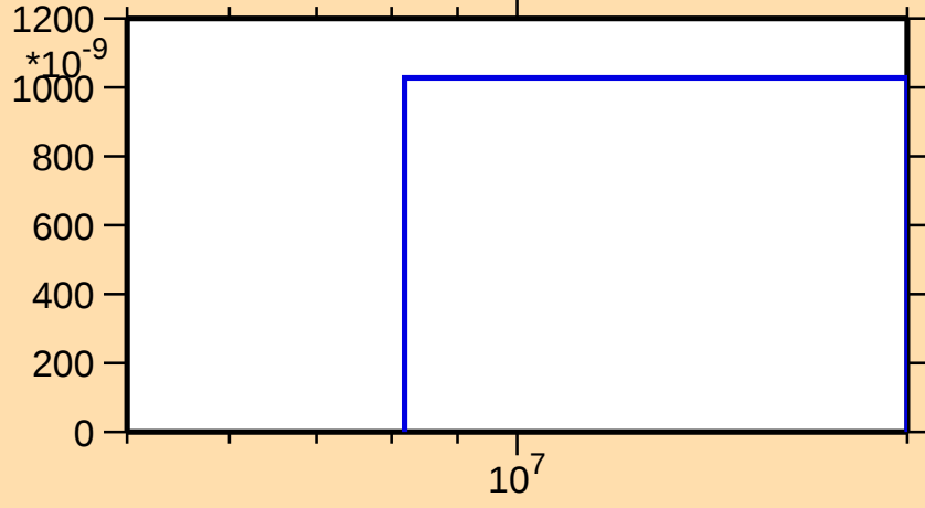
\sigma vs. E for ^{162}\text{Tm}(n,2n\alpha)
