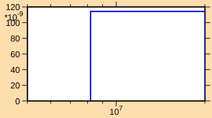
\sigma vs. E for ^{162}\text{Tm}(n,\text{He}3)
