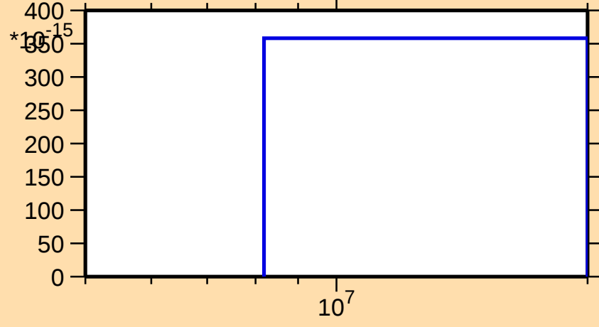
\sigma vs. E for ^{162}\text{Tm}(n,\text{pt})
