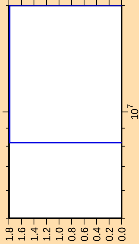
\Delta\sigma/\sigma vs. E for ^{162}\text{Tm}(n,\text{pt})
