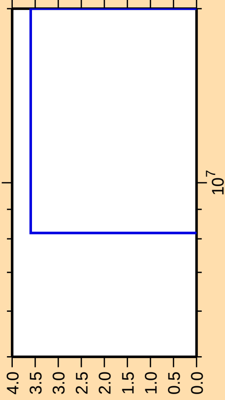
\Delta\sigma/\sigma vs. E for ^{162}\text{Tm} (mt 34)
