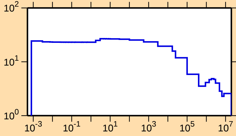
\sigma vs. E for ^{162}\text{Tm}(n,\text{el.})
