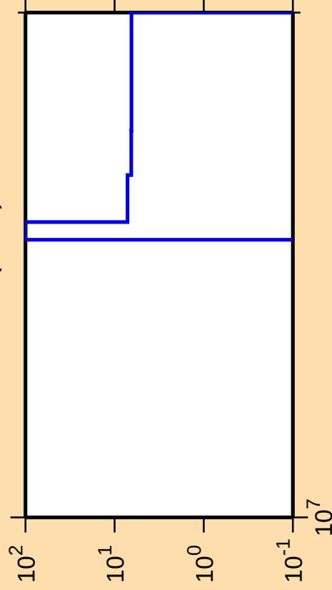
\Delta\sigma/\sigma vs. E for ^{170}\text{Tm}(n,3n)
