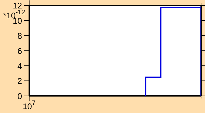
\sigma vs. E for ^{170}\text{Tm}(n,p\alpha)
