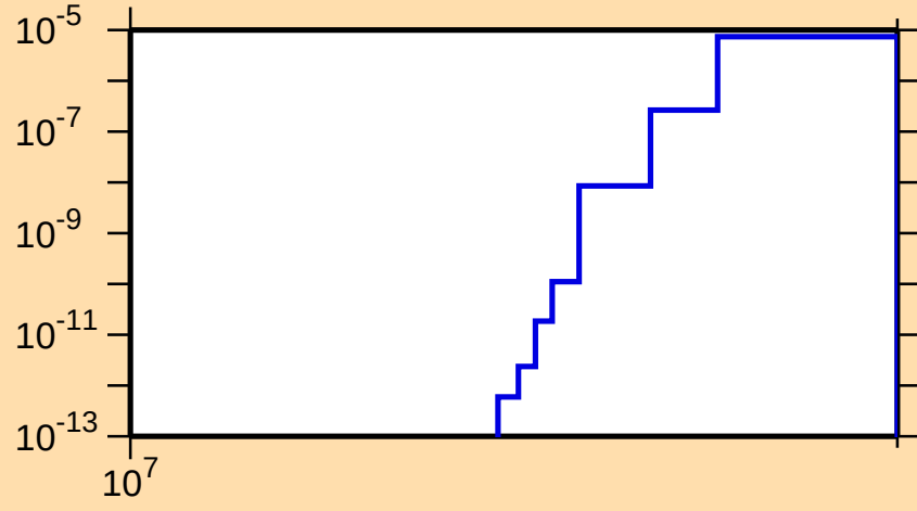
\sigma vs. E for ^{170}\text{Tm}(n,2np)
