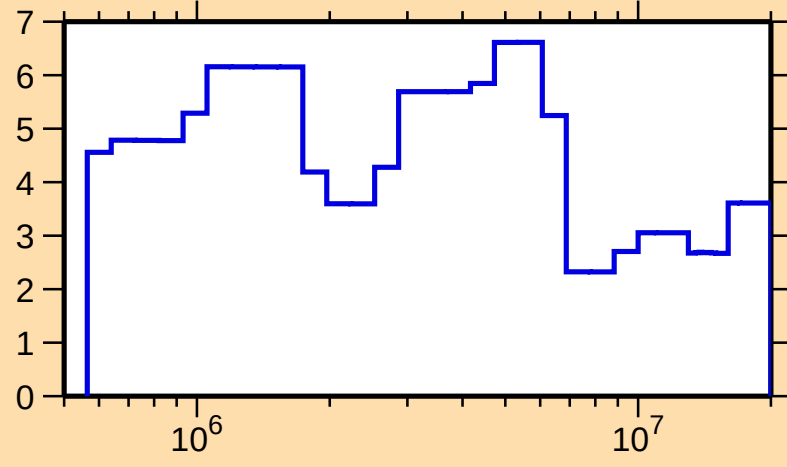
\Delta\sigma/\sigma vs. E for ^{170}\text{Tm}(n,\text{el.})
