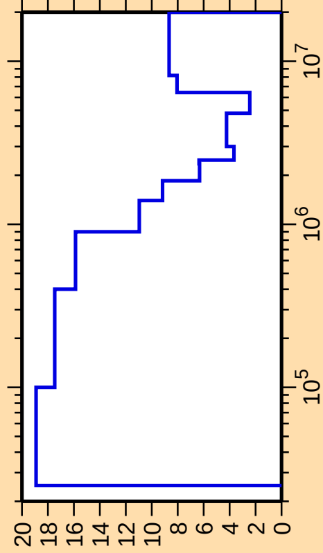
\Delta\sigma/\sigma vs. E for ^{170}\text{Tm}(n,\text{inel.})
