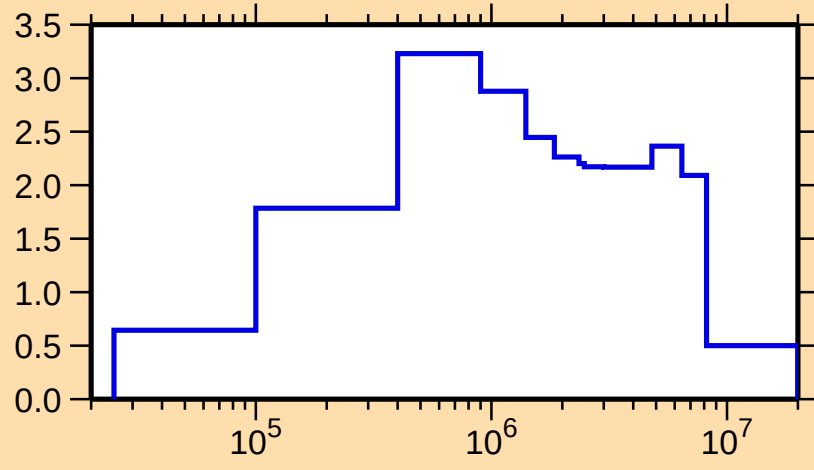
\sigma vs. E for ^{170}\text{Tm}(n,\text{inel.})
