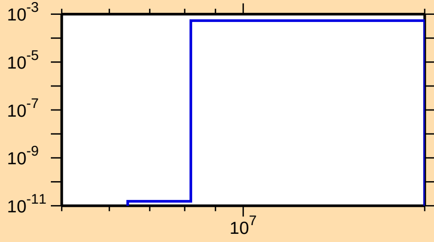
\sigma vs. E for ^{170}\text{Tm}(n,d)
