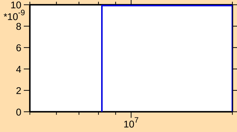
\sigma vs. E for ^{170}\text{Tm}(n,nt)
