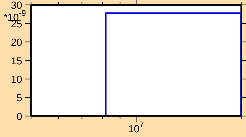
\sigma vs. E for ^{170}\text{Tm}(n,2n\alpha)
