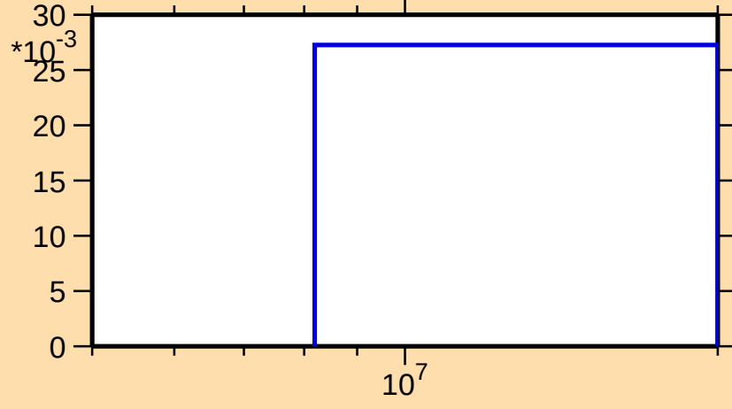
\sigma vs. E for ^{170}\text{Tm}(n,3n)
