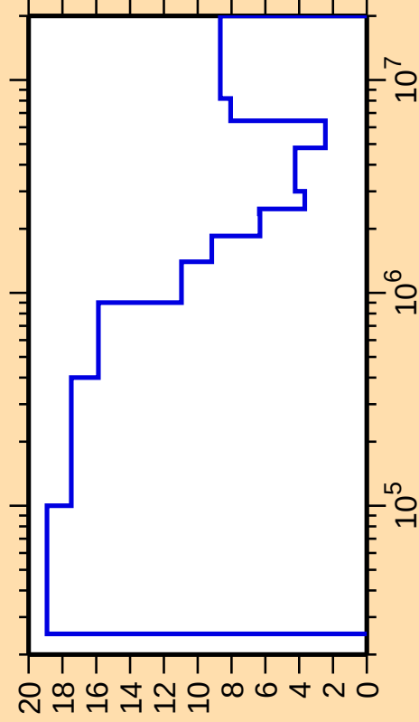
\Delta\sigma/\sigma vs. E for ^{170}\text{Tm}(n,\text{inel.})
