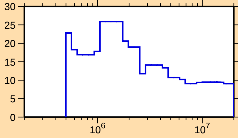
\Delta\sigma/\sigma vs. E for ^{230}\text{U}(\text{n},\text{nonel.})
