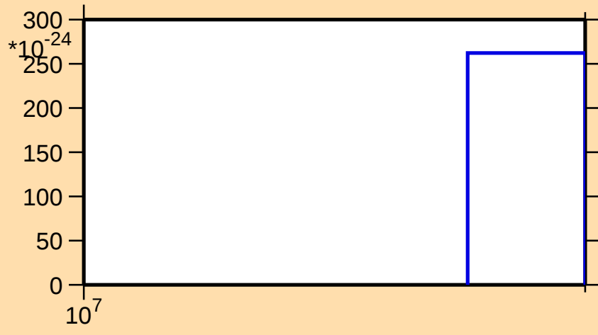
\sigma vs. E for ^{230}\text{U} (mt 42)
