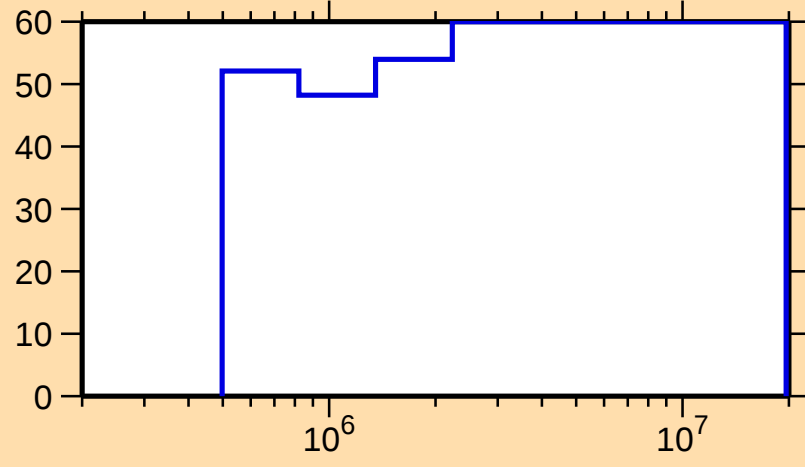
\Delta\sigma/\sigma vs. E for ^{230}\text{U}(\text{n},\text{inel.})
