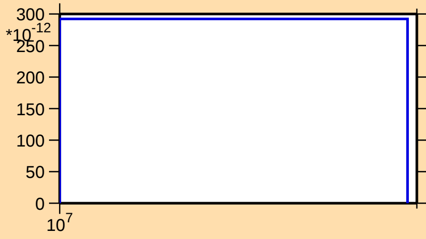
\sigma vs. E for ^{230}\text{U}(\text{n},\text{nd})
