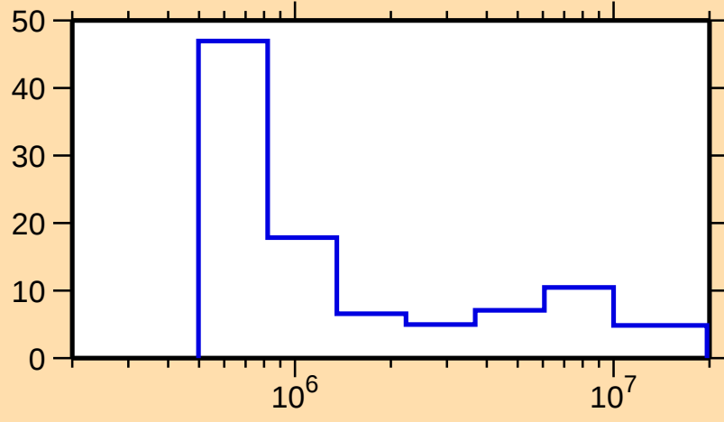
\Delta\sigma/\sigma vs. E for ^{230}\text{U}(\text{n,tot.})
