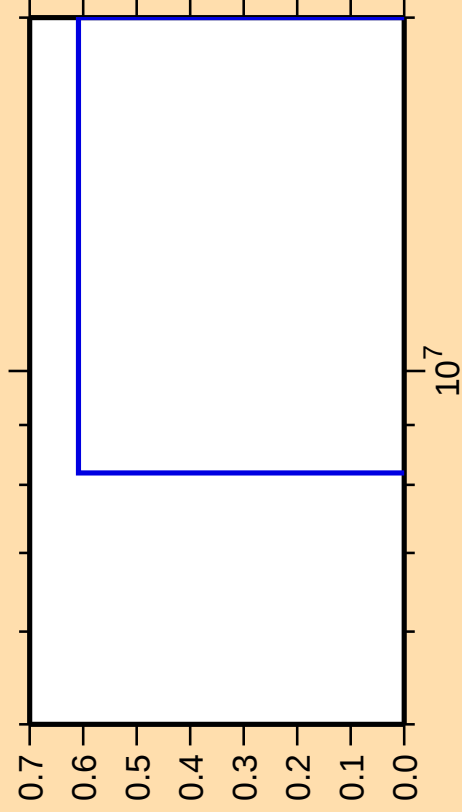
\Delta\sigma/\sigma vs. E for ^{230}\text{U}(n,nt)
