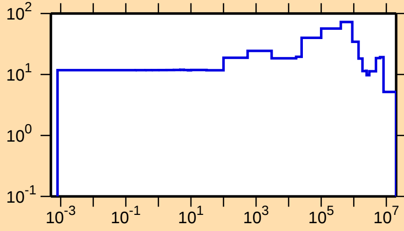
\Delta\sigma/\sigma vs. E for ^{230}\text{U}(\text{n,el.})
