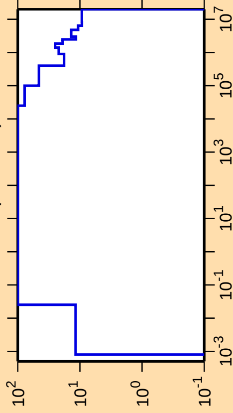
\Delta\sigma/\sigma vs. E for ^{230}\text{U}(n,\text{nonel.})
