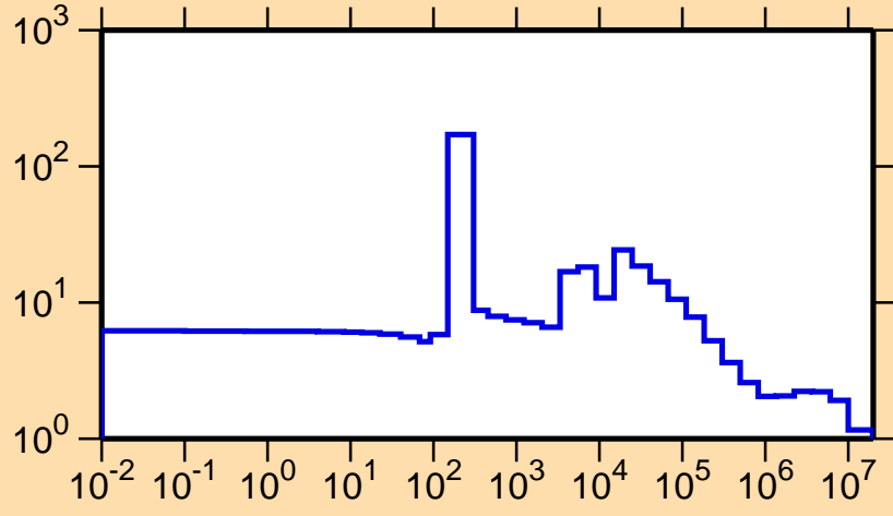
\sigma vs. E for ^{54}\text{V}(n,\text{el.})
