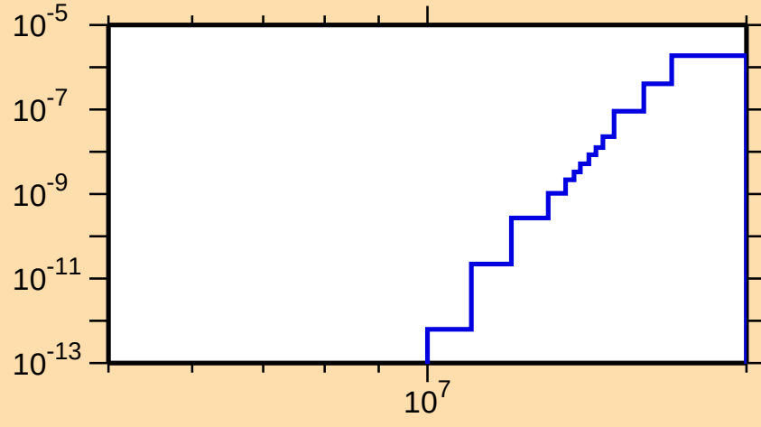
\sigma vs. E for ^{79}\text{Y}(\text{mt117})
