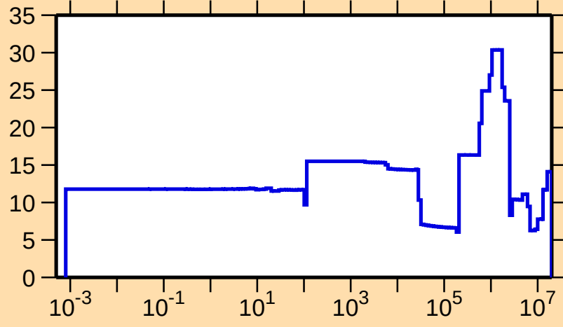
\Delta\sigma/\sigma vs. E for ^{79}\text{Y}(n,\text{el.})
