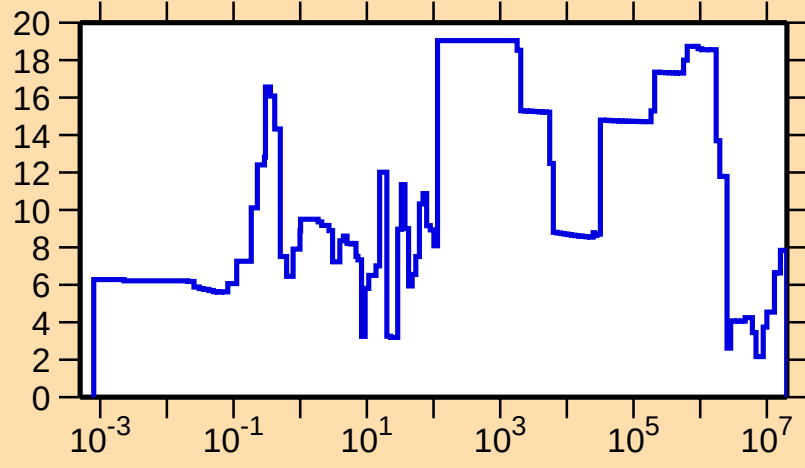
\Delta\sigma/\sigma vs. E for ^{79}\text{Y}(n,\text{tot.})
