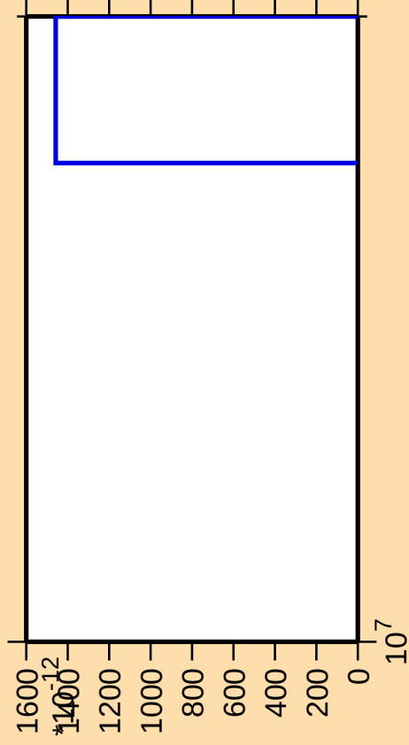
\Delta\sigma/\sigma vs. E for ^{79}\text{Y}(\text{n},\text{nt})
