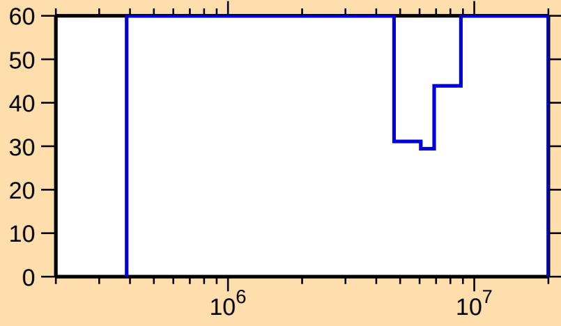
\Delta\sigma/\sigma vs. E for ^{79}\text{Y}(n,\text{ncont.})
