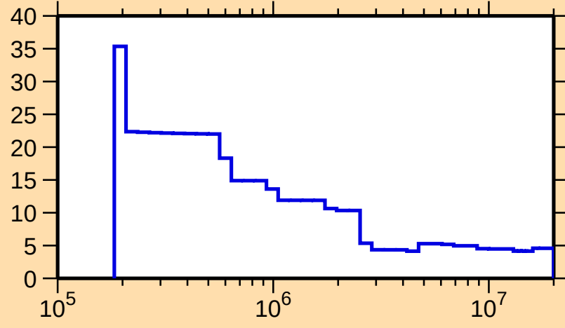
\Delta\sigma/\sigma vs. E for ^{79}\text{Y}(n,\text{nonel.})
