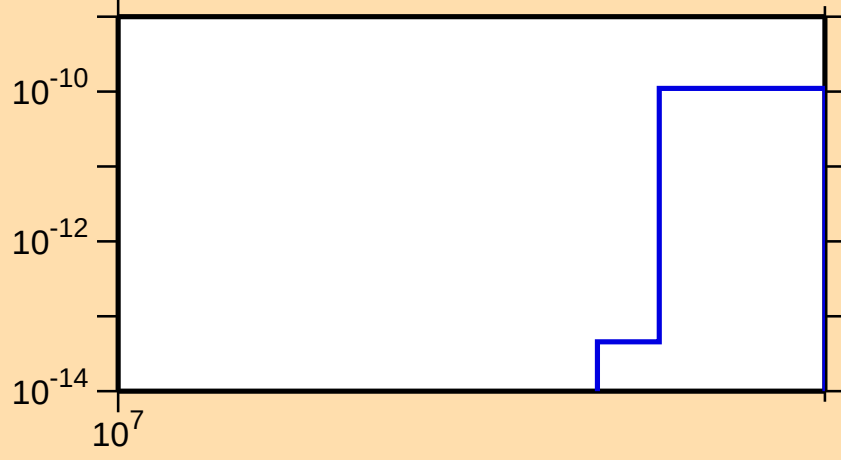
\sigma vs. E for ^{79}\text{Y} (mt 34)
