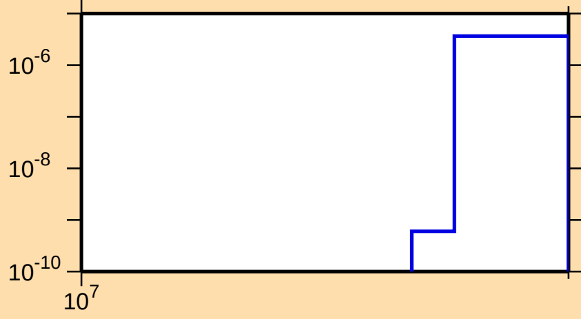
\sigma vs. E for ^{79}\text{Y}(n,2np)
