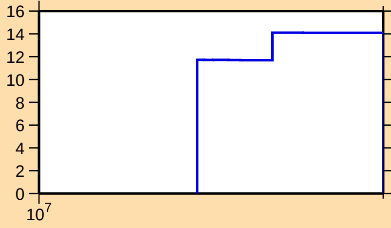
\Delta\sigma/\sigma vs. E for ^{79}\text{Y}(n,\text{el.})
