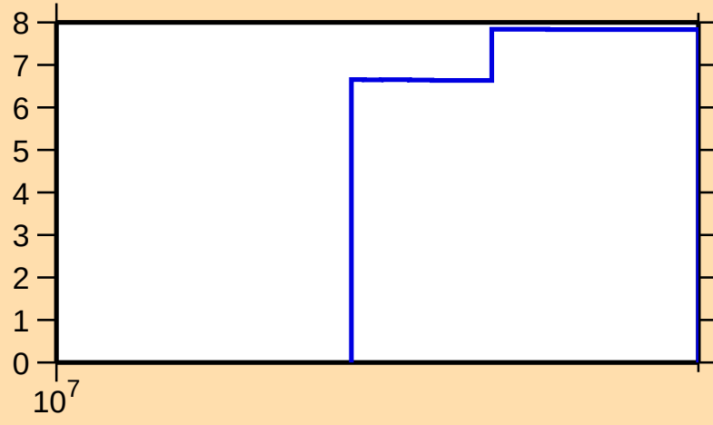
\Delta\sigma/\sigma vs. E for ^{79}\text{Y}(n,\text{tot.})
