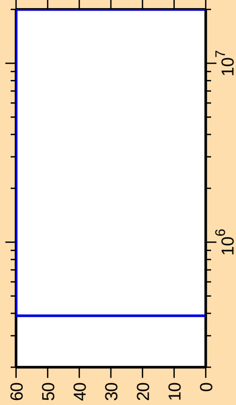
\Delta\sigma/\sigma vs. E for ^{79}\text{Y}(n,\alpha)
