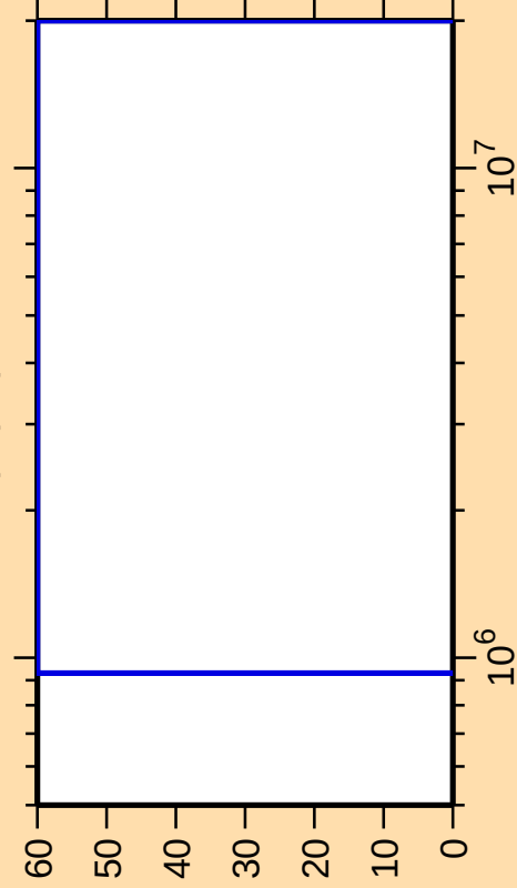
\Delta\sigma/\sigma vs. E for ^{79}\text{Y}(n,p\alpha)
