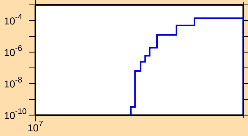
\sigma vs. E for ^{79}\text{Y}(n,2n)
