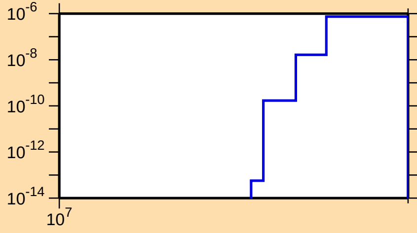
\sigma vs. E for ^{79}\text{Y}(n,\text{nd})
