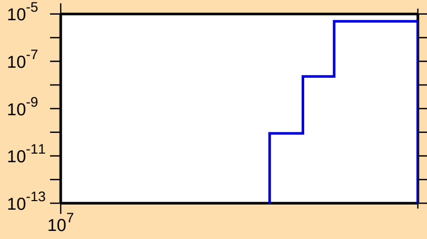
\sigma vs. E for ^{79}\text{Y}(n,\text{pt})
