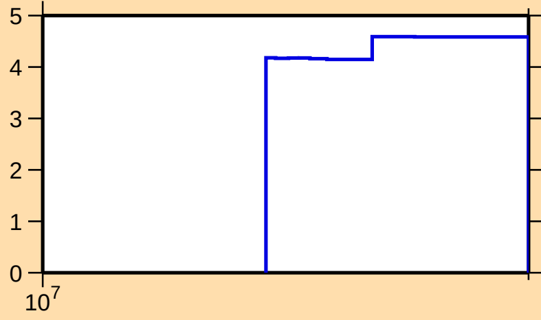
\Delta\sigma/\sigma vs. E for ^{79}\text{Y}(n,\text{nonel.})
