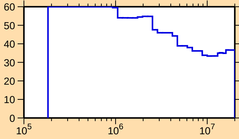
\Delta\sigma/\sigma vs. E for ^{79}\text{Y}(n,\text{inel.})
