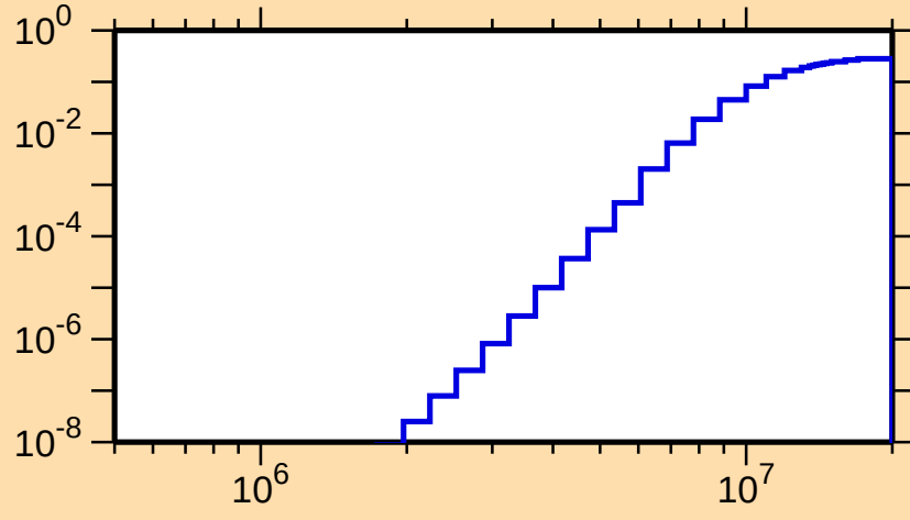
\sigma vs. E for ^{79}\text{Y}(n,p\alpha)
