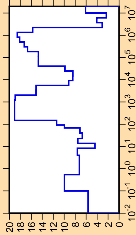
\Delta\sigma/\sigma vs. E for ^{79}\text{Y}(n,\text{tot.})
