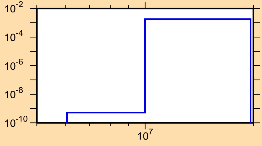
\sigma vs. E for ^{79}\text{Y}(n,\text{pd})
