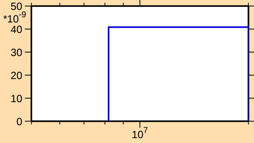
\sigma vs. E for ^{79}\text{Y}(n,\text{pt})
