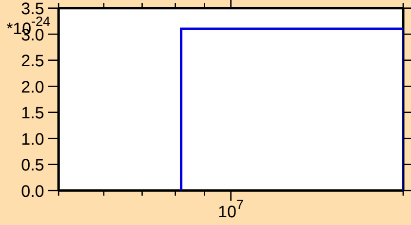
\sigma vs. E for ^{79}\text{Y}(\text{n},\text{nt})
