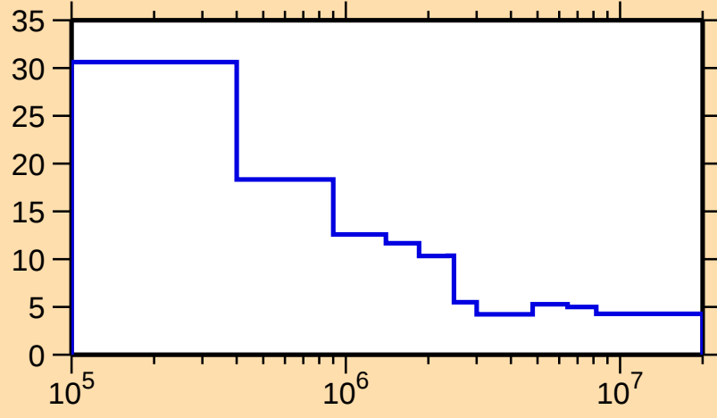
\Delta\sigma/\sigma vs. E for ^{79}\text{Y}(n,\text{nonel.})
