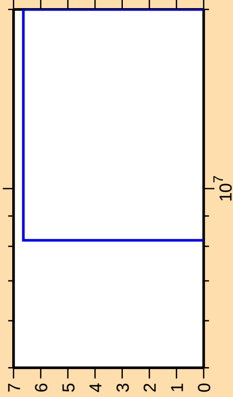
\Delta\sigma/\sigma vs. E for ^{79}\text{Y} (mt 34)
