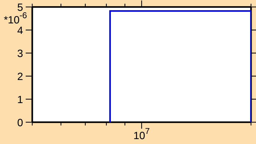
\sigma vs. E for ^{79}\text{Y}(n,2n)
