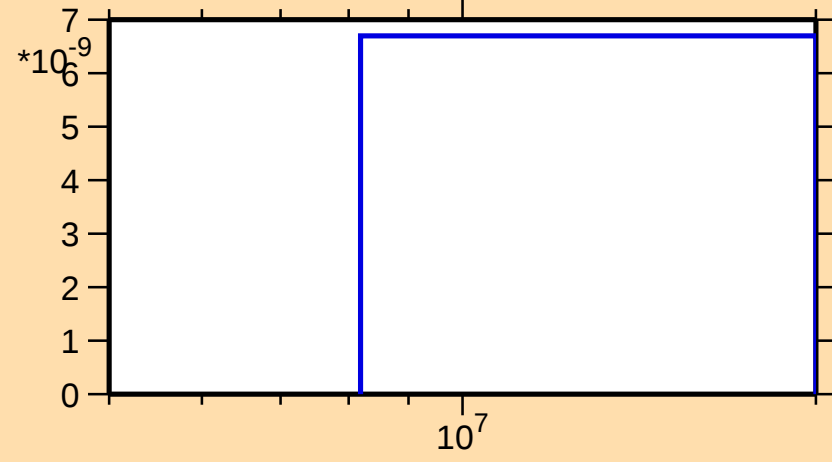
\sigma vs. E for ^{79}\text{Y}(\text{n},\text{nd})
