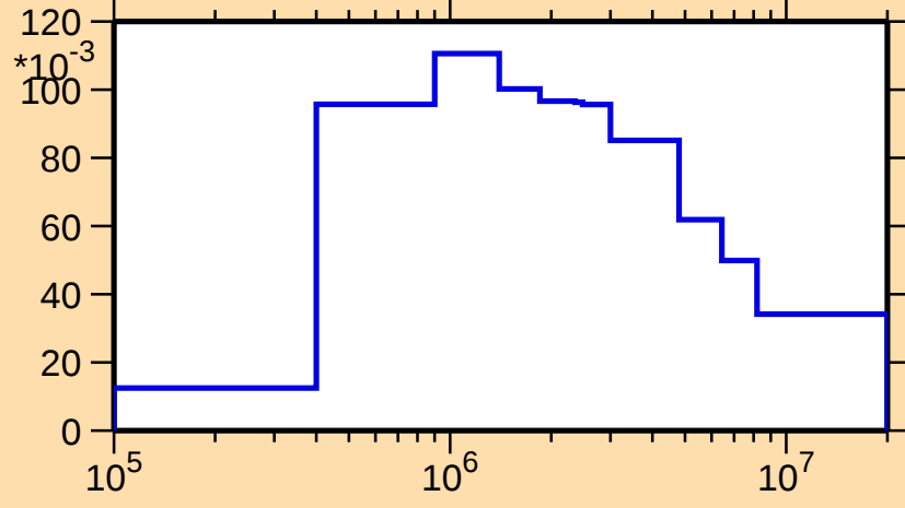
\sigma vs. E for ^{79}\text{Y}(n,n_1)
