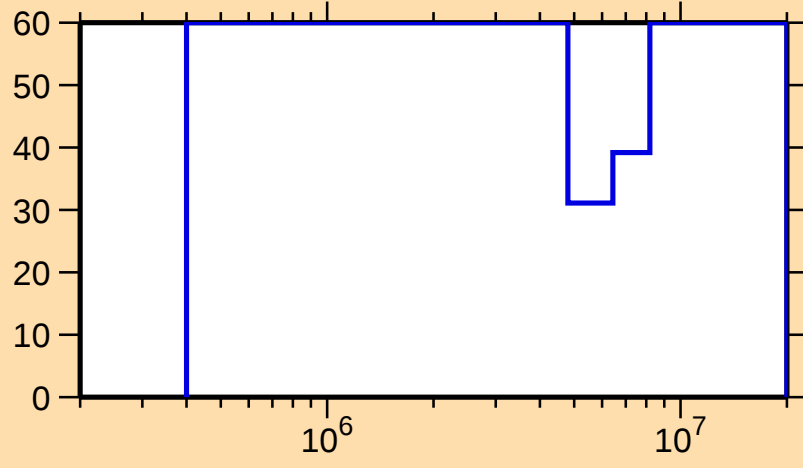
\Delta\sigma/\sigma vs. E for ^{79}\text{Y}(n,n\text{cont.})
