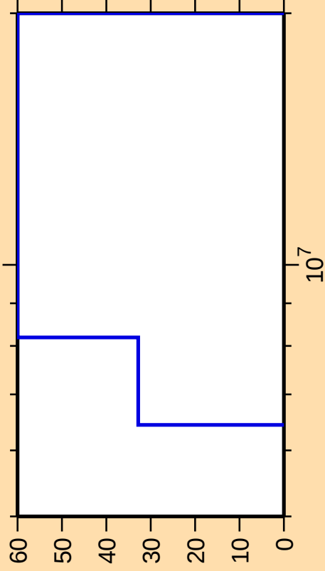
\Delta\sigma/\sigma vs. E for ^{79}\text{Y}(n,n\alpha)
