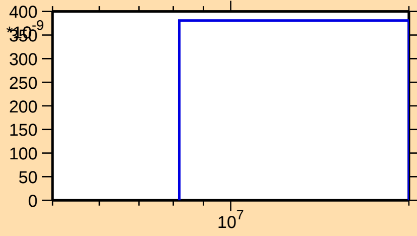
\sigma vs. E for ^{79}\text{Y} (mt 45)
