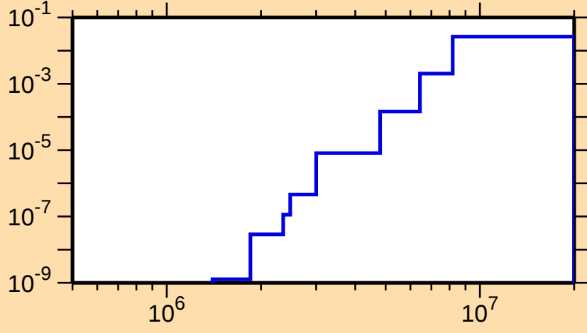
\sigma vs. E for ^{79}\text{Y}(n,d)
