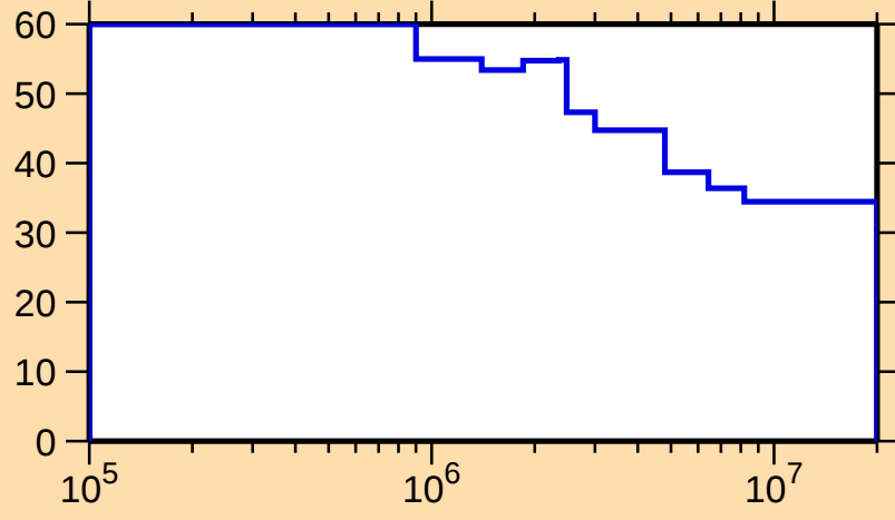
\Delta\sigma/\sigma vs. E for ^{79}\text{Y}(n,n_1)
