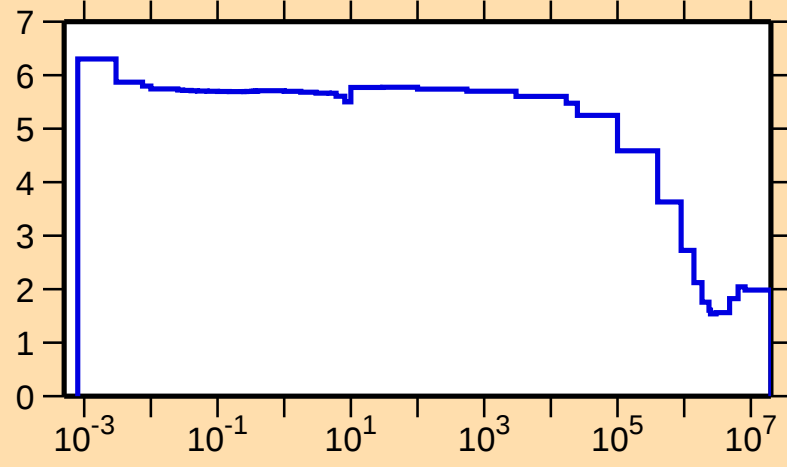
\sigma vs. E for ^{79}\text{Y}(n,\text{el.})
