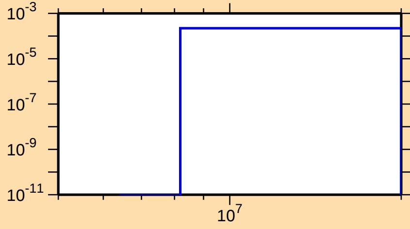
\sigma vs. E for ^{79}\text{Y}(n,n\alpha)
