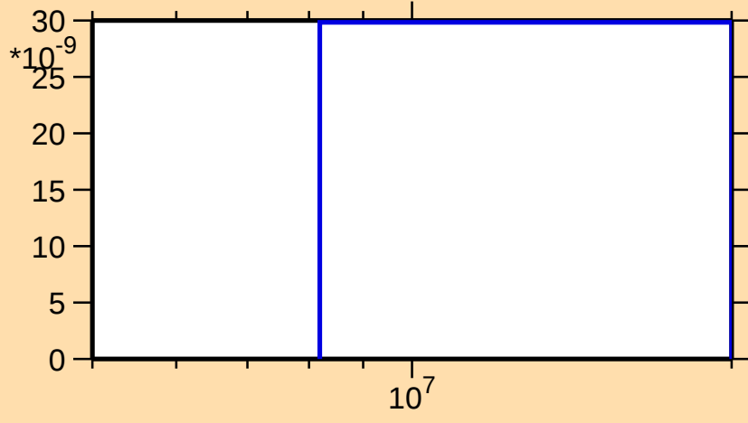
\sigma vs. E for ^{79}\text{Y}(n,2np)
