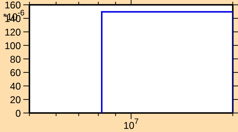
\sigma vs. E for ^{79}\text{Y}(n,t)
