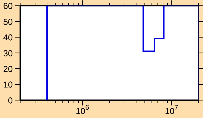
\Delta\sigma/\sigma vs. E for ^{79}\text{Y}(n,n\text{cont.})
