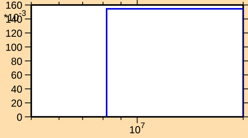
\sigma vs. E for ^{85}\text{Y}(n,2n)
