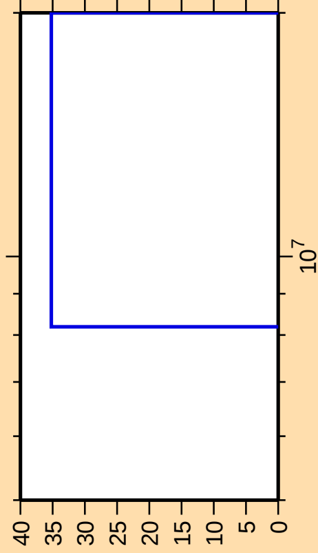
\Delta\sigma/\sigma vs. E for ^{85}\text{Y}(\text{mt } 45)
