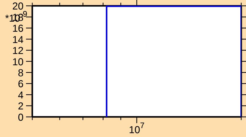
\sigma vs. E for ^{85}\text{Y}(n,\text{pd})
