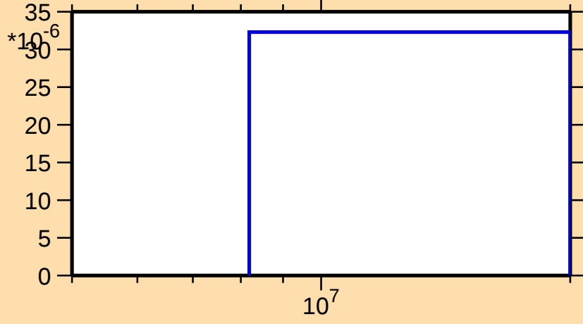
\sigma vs. E for ^{85}\text{Y}(n,t)
