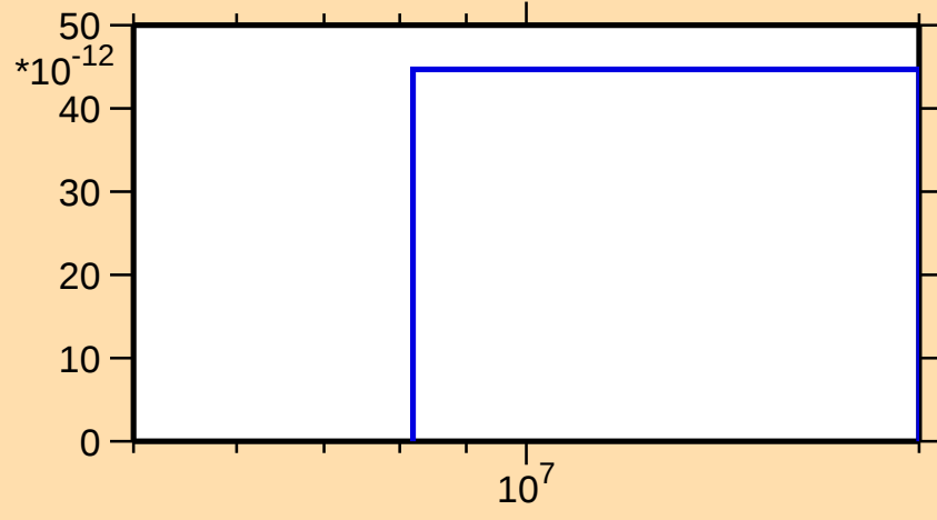
\sigma vs. E for ^{85}\text{Y}(\text{mt } 45)
