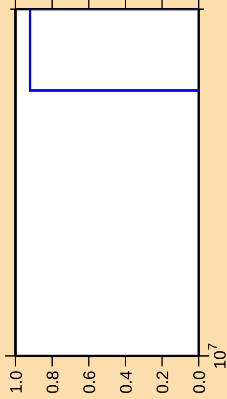
\Delta\sigma/\sigma vs. E for ^{87}\text{Y}(\text{n},\text{nt})
