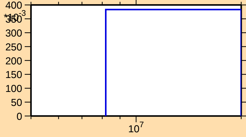
\sigma vs. E for ^{87}\text{Y}(n,2n)
