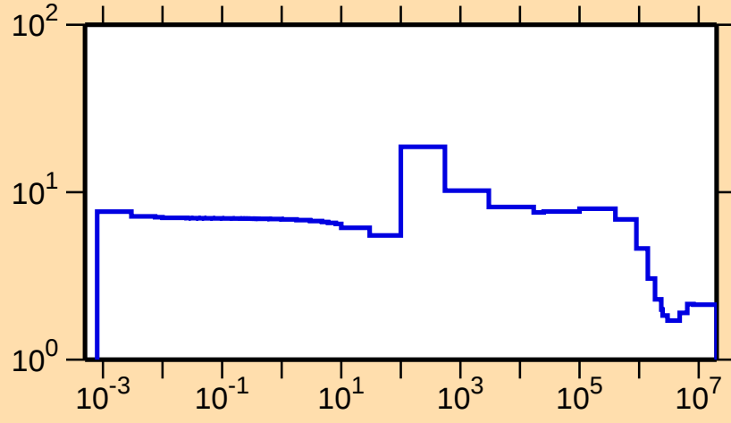
\sigma vs. E for ^{87}\text{Y}(n,\text{el.})
