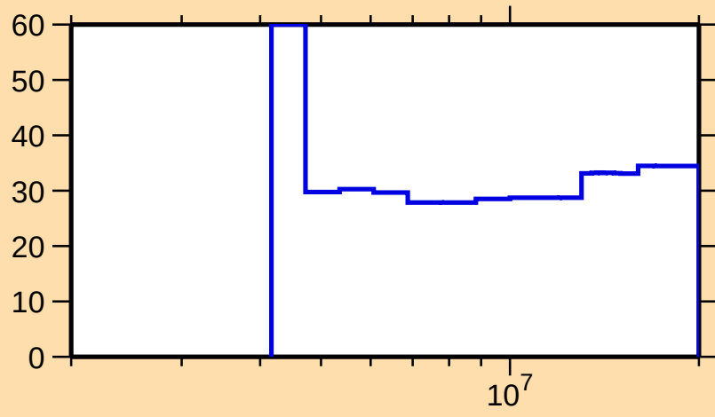
\Delta\sigma/\sigma vs. E for ^{96}\text{Y}(n,n_1)
