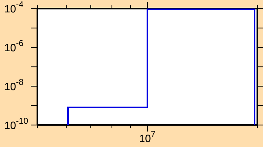
\sigma vs. E for ^{96}\text{Y}(n,t)
