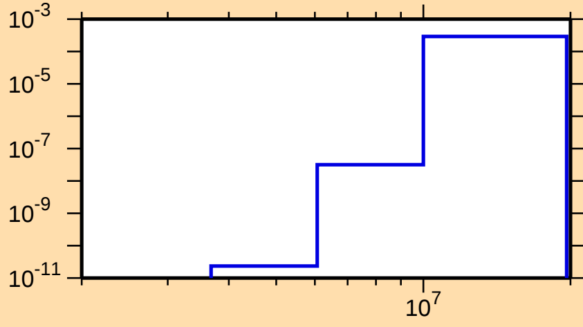
\sigma vs. E for ^{96}\text{Y}(n,\alpha)
