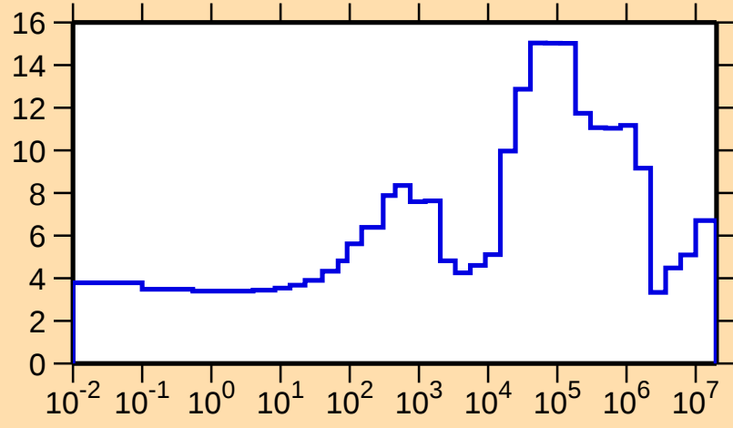
\Delta\sigma/\sigma vs. E for ^{96}\text{Y}(\text{n,tot.})
