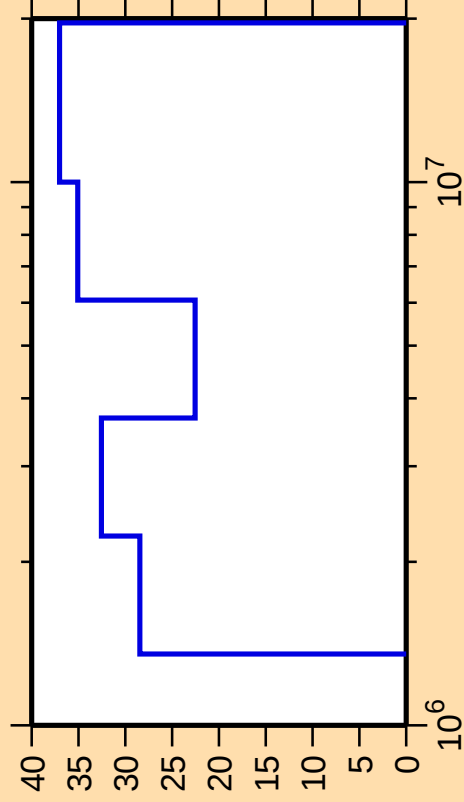
\Delta\sigma/\sigma vs. E for ^{96}\text{Y}(n,\gamma)
