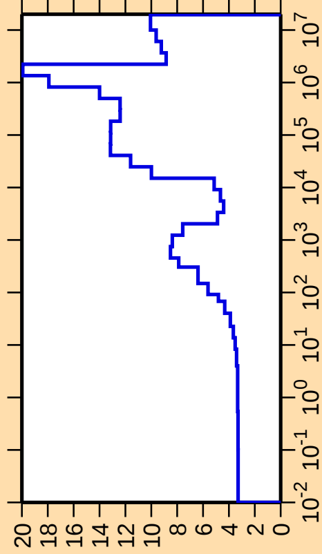
\Delta\sigma/\sigma vs. E for ^{96}\text{Y}(\text{n,el.})
