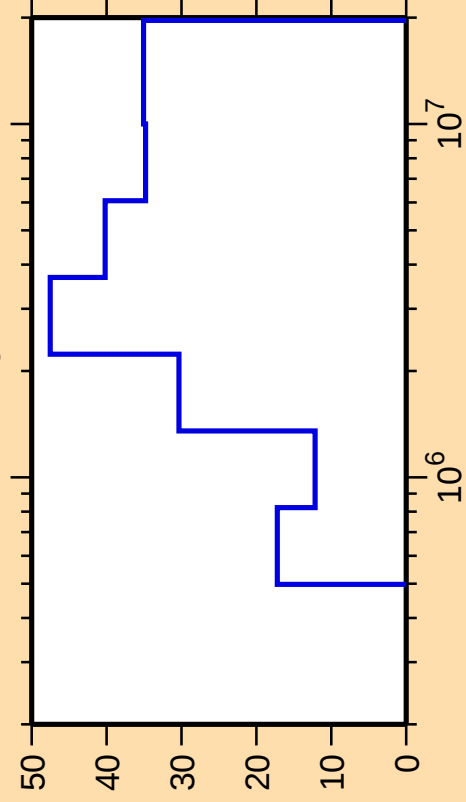
\Delta\sigma/\sigma vs. E for ^{96}\text{Y}(n,n_3)
