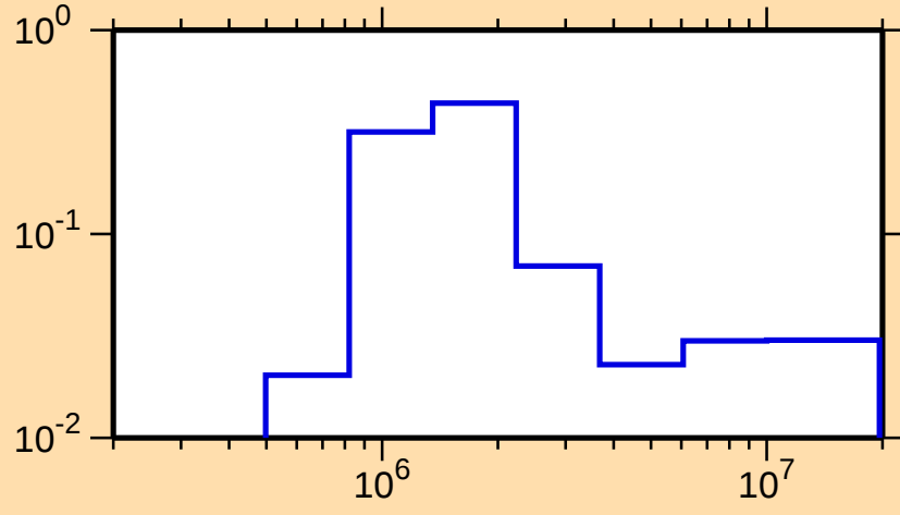
\sigma vs. E for ^{96}\text{Y}(n,n_3)
