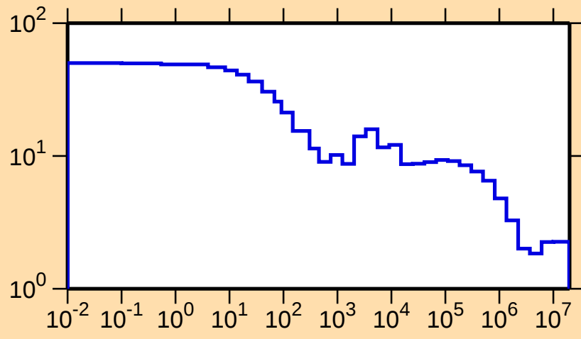
\sigma vs. E for ^{96}\text{Y}(n,\text{el.})
