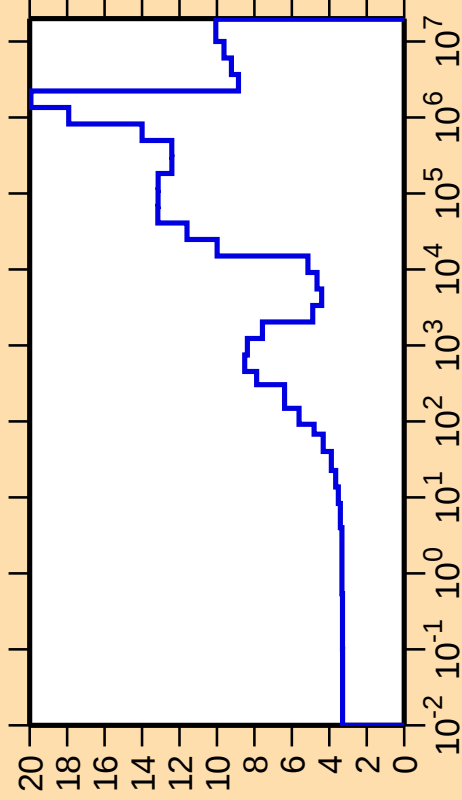
\Delta\sigma/\sigma vs. E for ^{96}\text{Y}(n,\text{el.})
