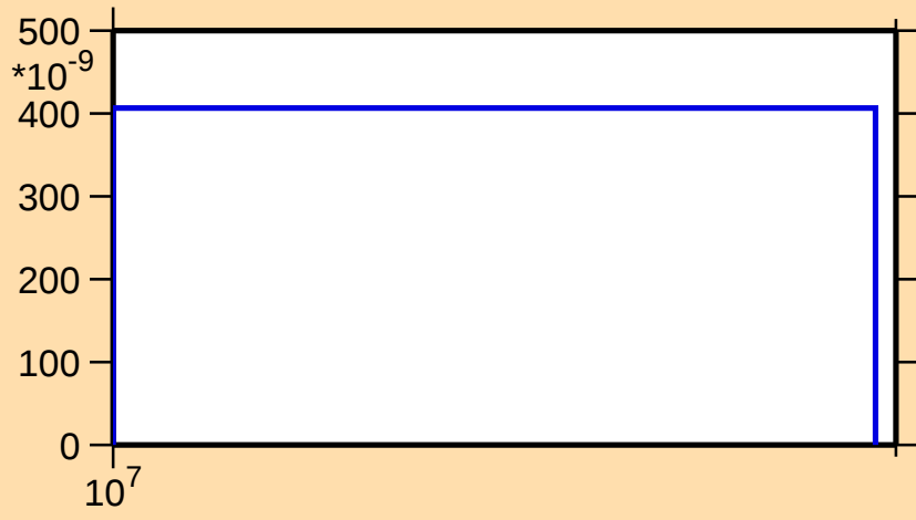
\sigma vs. E for ^{96}\text{Y}(n,\text{nd})
