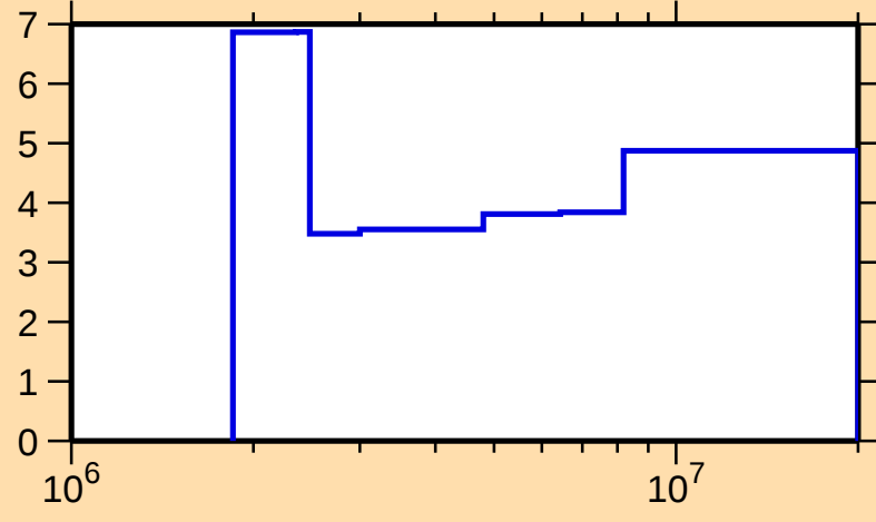
\Delta\sigma/\sigma vs. E for ^{96}\text{Y}(n,n\text{onel.})
