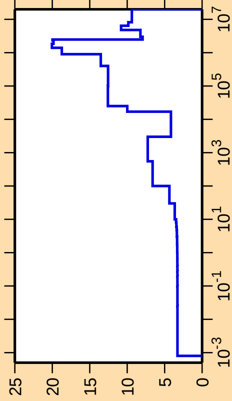
\Delta\sigma/\sigma vs. E for ^{96}\text{Y}(\text{n},\text{el.})
