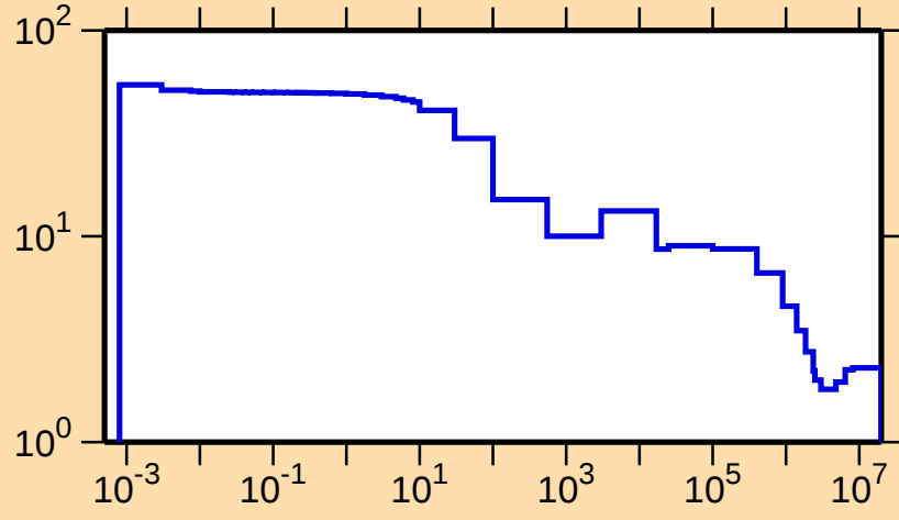
\sigma vs. E for ^{96}\text{Y}(\text{n},\text{el.})
