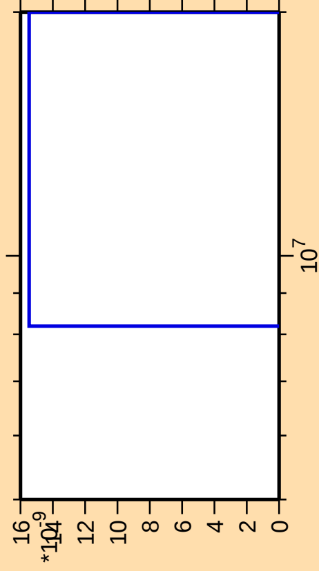
\Delta\sigma/\sigma vs. E for ^{96}\text{Y}(\text{mt } 11)
