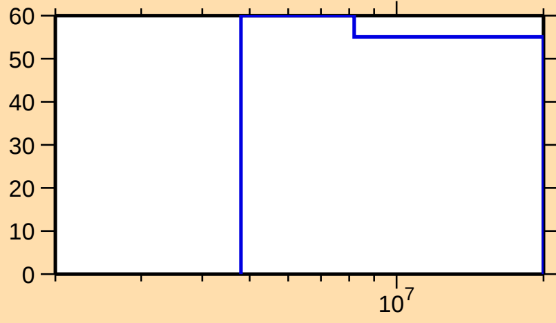
\Delta\sigma/\sigma vs. E for ^{96}\text{Y}(n,p)
