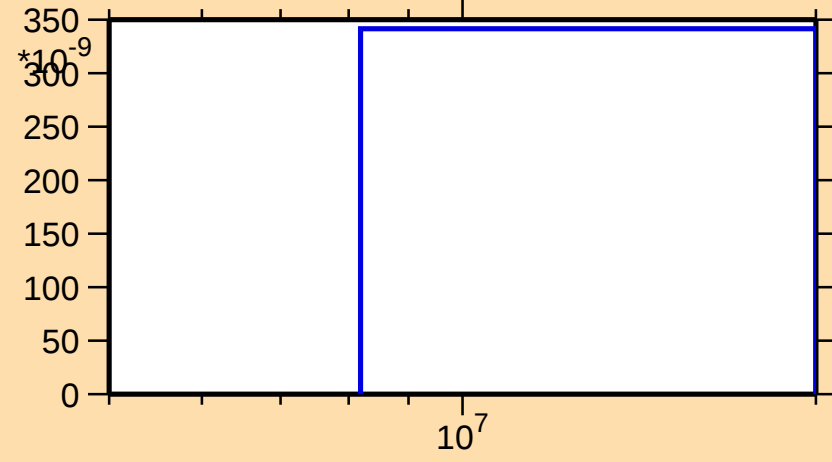
\sigma vs. E for ^{96}\text{Y}(\text{n},\text{nd})
