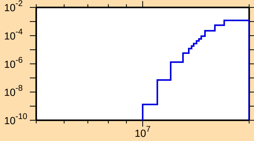
\sigma vs. E for ^{151}\text{Yb}(n,t)
