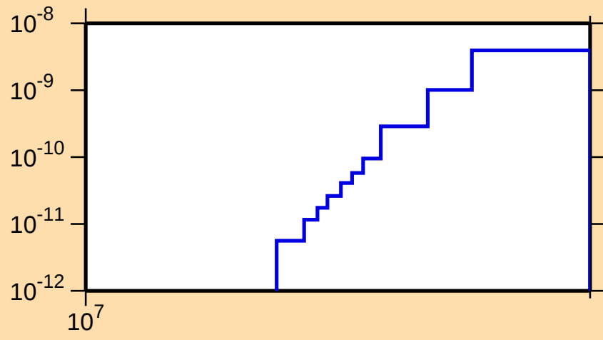
\sigma vs. E for ^{152}\text{Yb}(\text{mt117})
