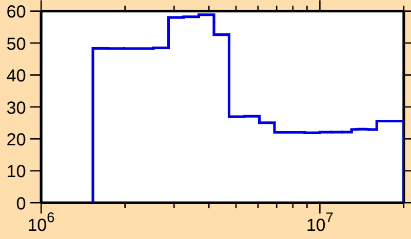
\Delta\sigma/\sigma vs. E for ^{152}\text{Yb}(n,n_1)
