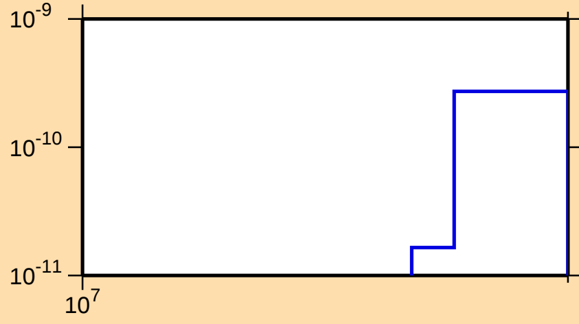
\sigma vs. E for ^{152}\text{Yb} (mt 34)
