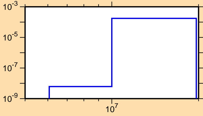
\sigma vs. E for ^{152}\text{Yb}(n,\text{pd})
