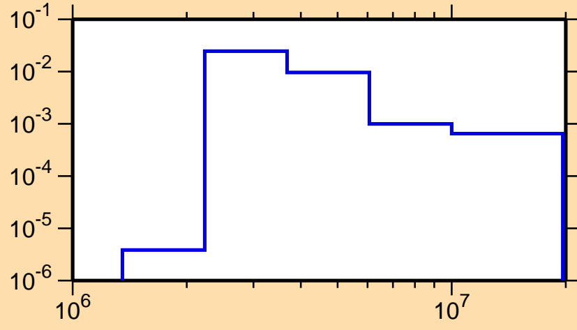
\sigma vs. E for ^{152}\text{Yb}(n,n_3)
