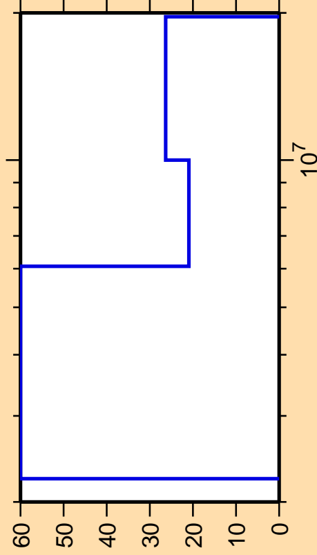
\Delta\sigma/\sigma vs. E for ^{152}\text{Yb}(n,n_4)
