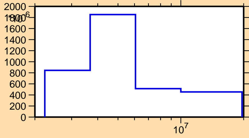
\sigma vs. E for ^{152}\text{Yb}(n,n_4)
