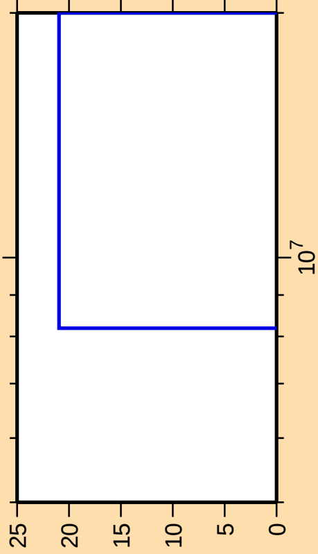
\Delta\sigma/\sigma vs. E for ^{152}\text{Yb}(\text{mt } 34)
