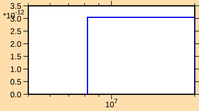
\sigma vs. E for ^{152}\text{Yb}(\text{mt } 34)
