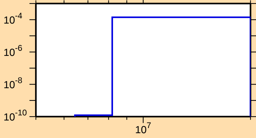
\sigma vs. E for ^{152}\text{Yb}(n,\text{pd})
