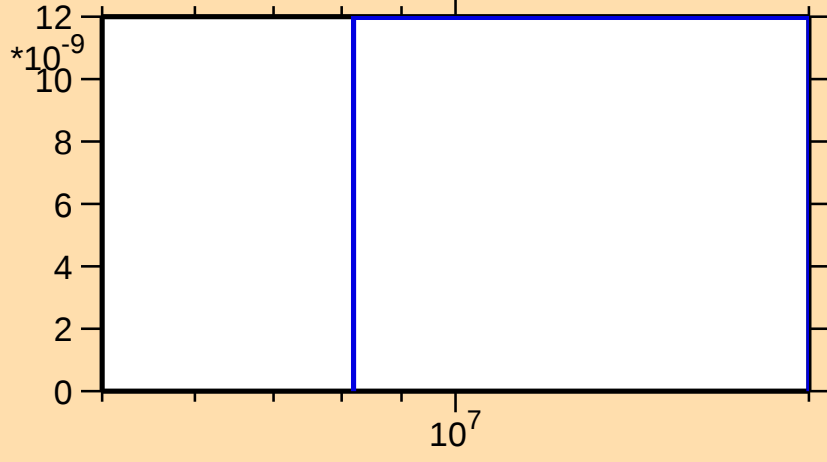
\sigma vs. E for ^{152}\text{Yb}(n,\text{pt})
