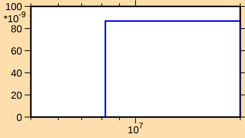
\sigma vs. E for ^{152}\text{Yb}(\text{mt } 45)
