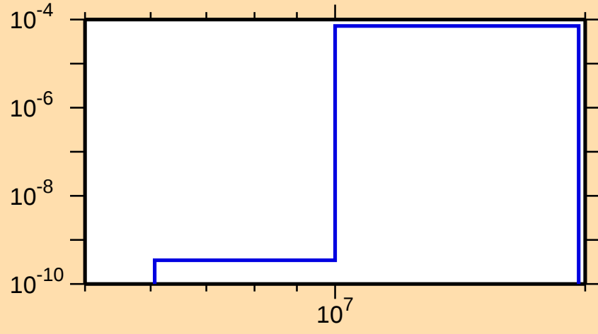
\sigma vs. E for ^{153}\text{Yb}(n,\text{pd})
