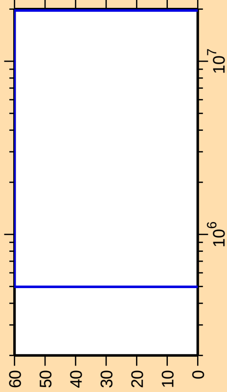
\Delta\sigma/\sigma vs. E for ^{153}\text{Yb}(n,\text{inel.})
