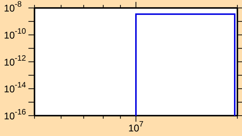
\sigma vs. E for ^{153}\text{Yb}(\text{mt } 34)
