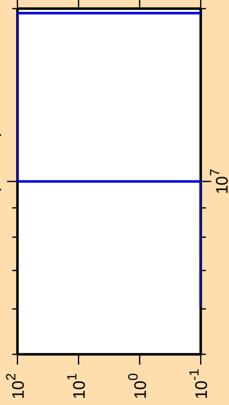
\Delta\sigma/\sigma vs. E for ^{153}\text{Yb}(\text{mt } 34)
