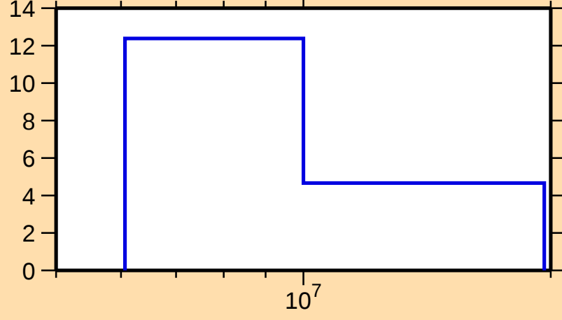
\Delta\sigma/\sigma vs. E for ^{153}\text{Yb}(n,\text{tot.})
