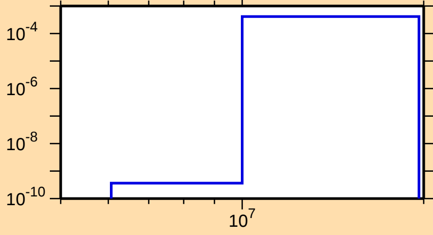
\sigma vs. E for ^{153}\text{Yb}(n,t)
