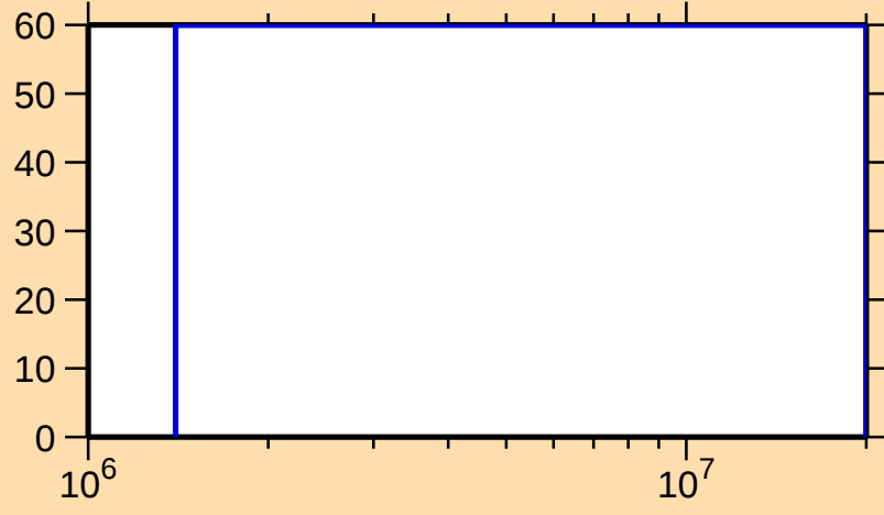
\Delta\sigma/\sigma vs. E for ^{153}\text{Yb}(n,n_1)
