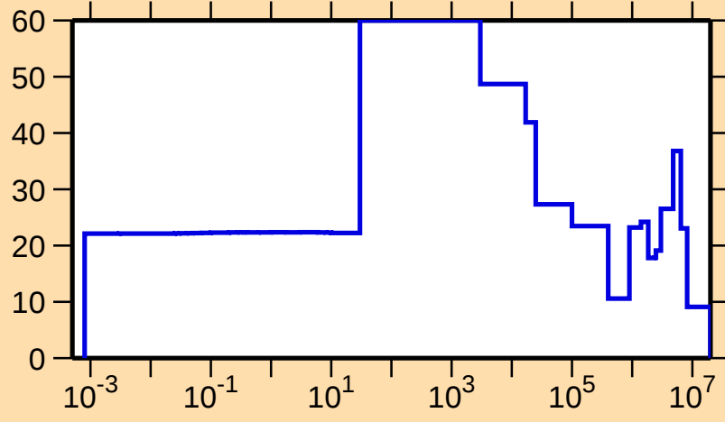
\Delta\sigma/\sigma vs. E for ^{153}\text{Yb}(n,\text{el.})
