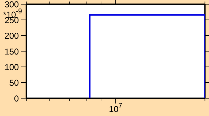
\sigma vs. E for ^{153}\text{Yb}(n,\text{nd})
