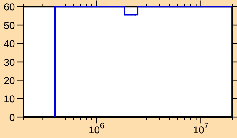
\Delta\sigma/\sigma vs. E for ^{153}\text{Yb}(n,\text{inel.})
