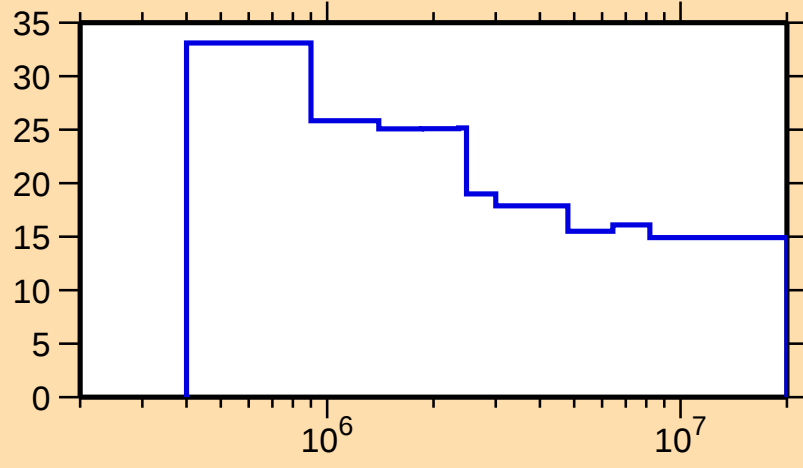
\Delta\sigma/\sigma vs. E for ^{153}\text{Yb}(n,\text{nonel.})
