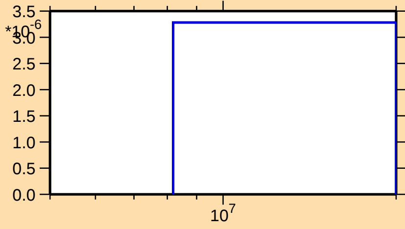
\sigma vs. E for ^{153}\text{Yb}(n,\text{pt})
