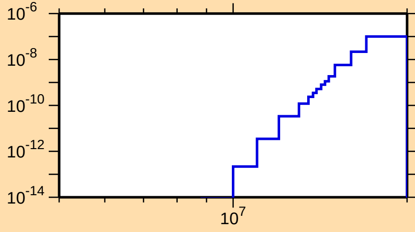
\sigma vs. E for ^{157}\text{Yb}(\text{mt117})
