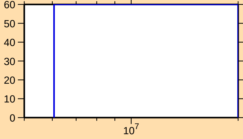
\Delta\sigma/\sigma vs. E for ^{157}\text{Yb}(n,n_1)
