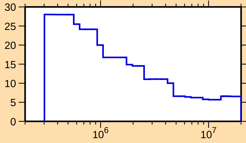
\Delta\sigma/\sigma vs. E for ^{157}\text{Yb}(n,\text{nonel.})
