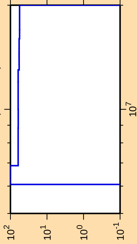
\Delta\sigma/\sigma vs. E for ^{157}\text{Yb}(n,\text{ncont.})
