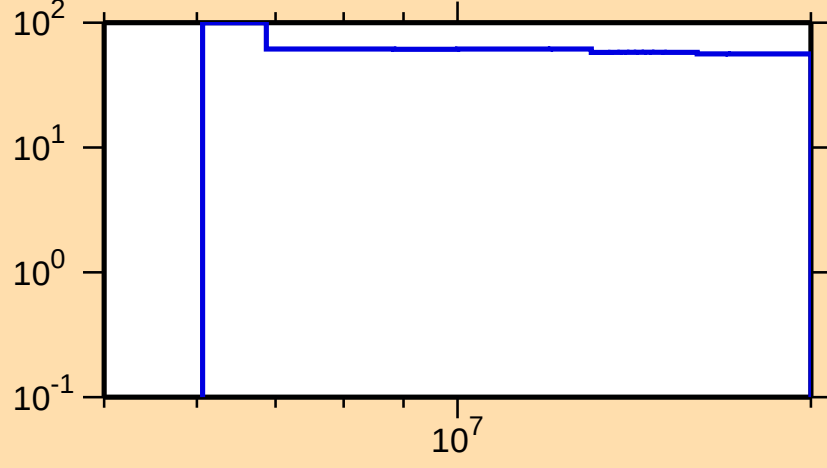
\Delta\sigma/\sigma vs. E for ^{157}\text{Yb}(n,n\text{cont.})
