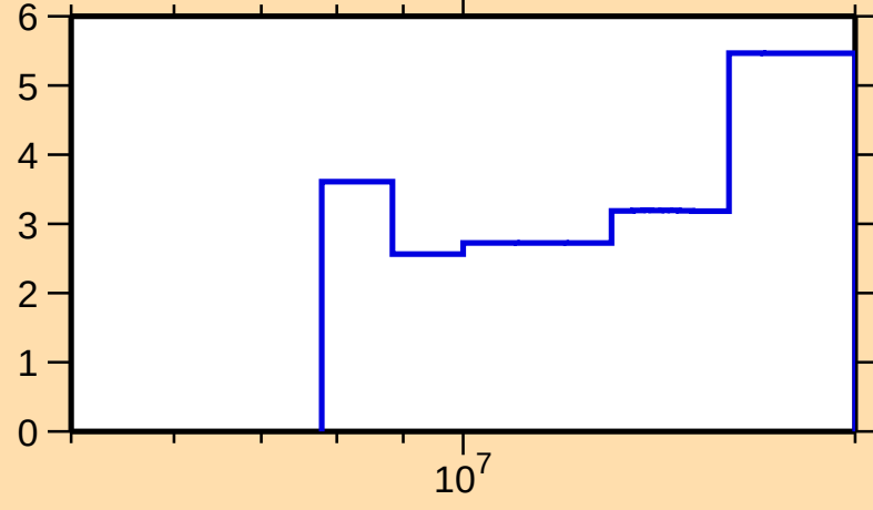
\Delta\sigma/\sigma vs. E for ^{157}\text{Yb}(n,\text{tot.})
