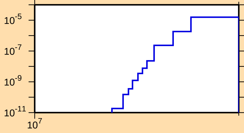
\sigma vs. E for ^{157}\text{Yb}(n,\text{nd})
