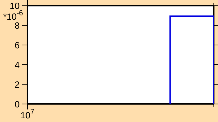
\sigma vs. E for ^{157}\text{Yb}(n,3n)
