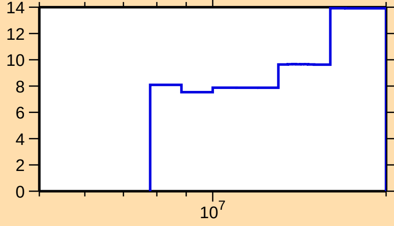
\Delta\sigma/\sigma vs. E for ^{157}\text{Yb}(n,\text{el.})
