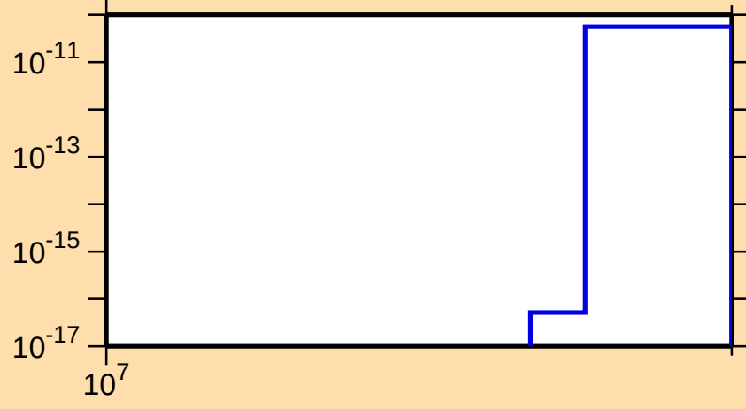
\sigma vs. E for ^{157}\text{Yb}(n,nt)
