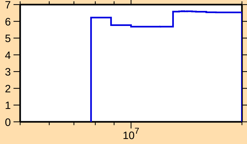
\Delta\sigma/\sigma vs. E for ^{157}\text{Yb}(n,\text{nonel.})
