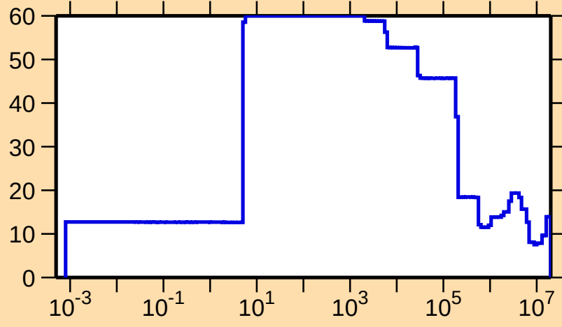
\Delta\sigma/\sigma vs. E for ^{157}\text{Yb}(n,\text{el.})
