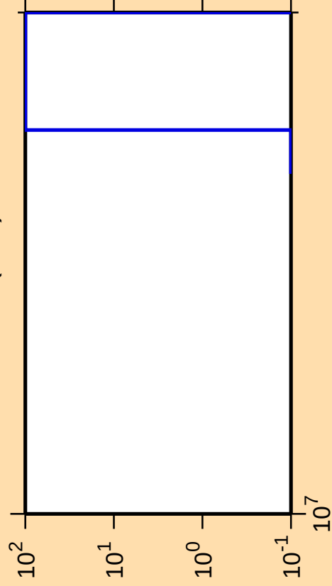
\Delta\sigma/\sigma vs. E for ^{157}\text{Yb}(n,nt)
