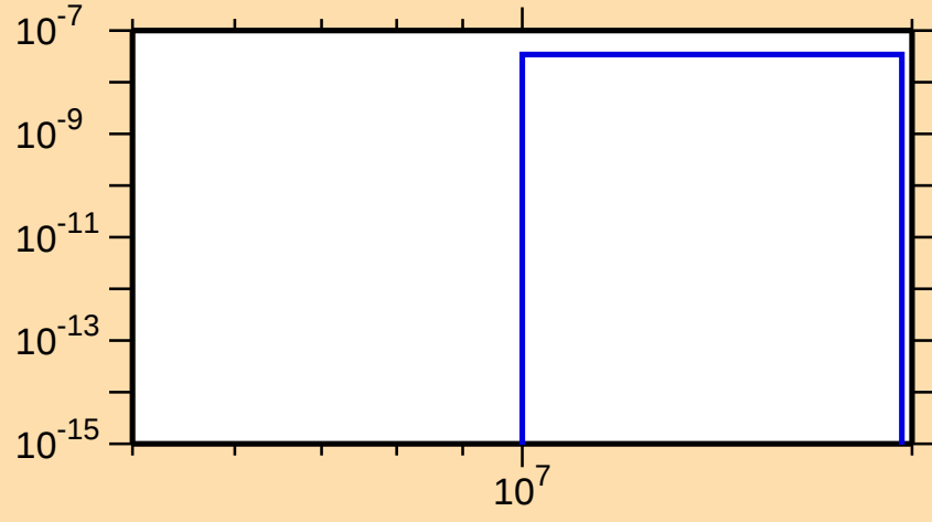
\sigma vs. E for ^{157}\text{Yb}(n,\text{pt})
