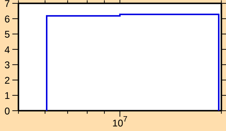
\Delta\sigma/\sigma vs. E for ^{157}\text{Yb}(n,\text{nonel.})
