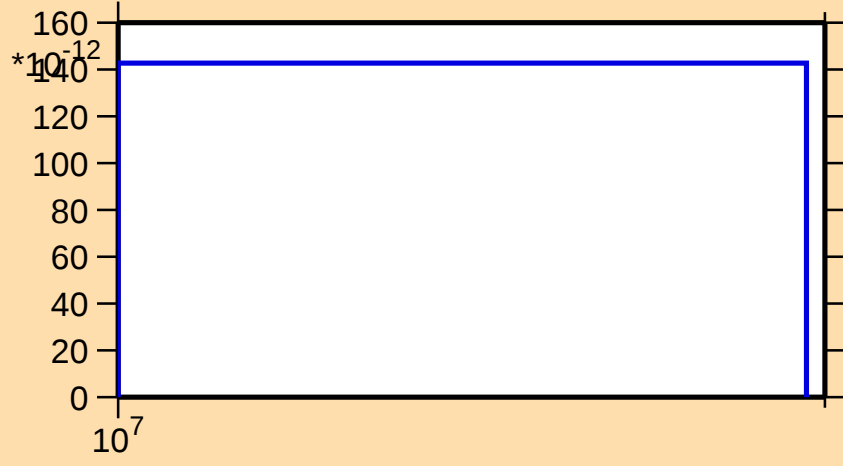
\sigma vs. E for ^{157}\text{Yb} (mt 34)
