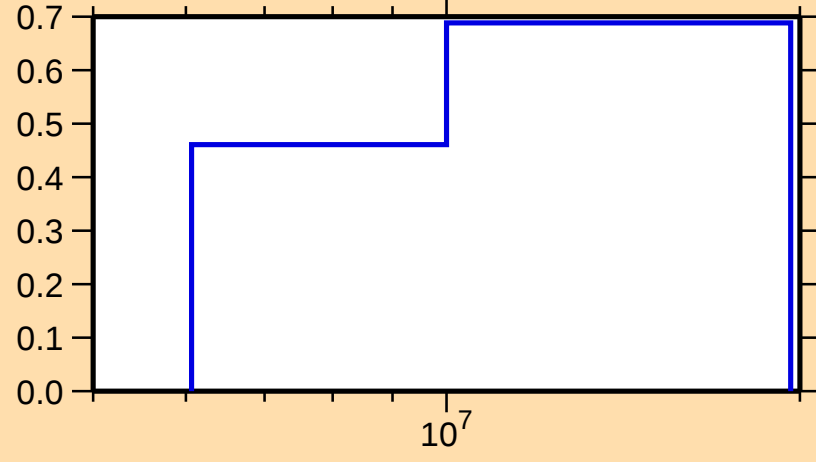
\sigma vs. E for ^{157}\text{Yb}(n,n\text{cont.})
