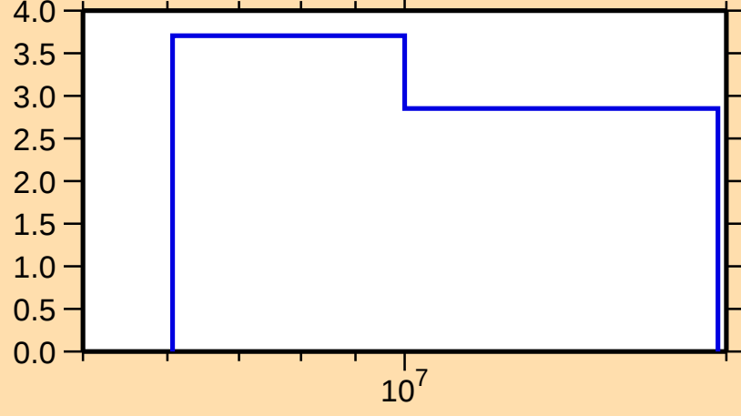
\Delta\sigma/\sigma vs. E for ^{157}\text{Yb}(n,\text{tot.})
