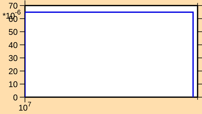
\sigma vs. E for ^{157}\text{Yb}(n,2np)
