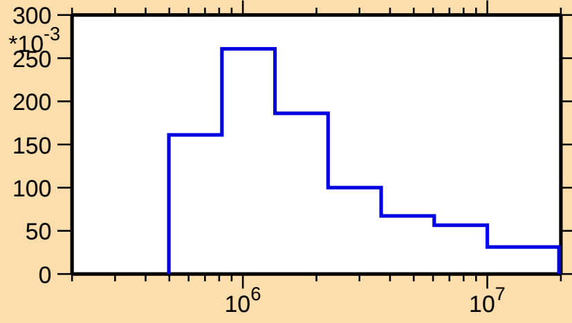
\sigma vs. E for ^{157}\text{Yb}(n,n_2)
