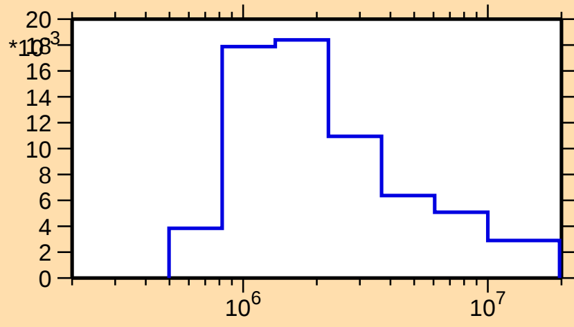
\sigma vs. E for ^{157}\text{Yb}(n,n_3)
