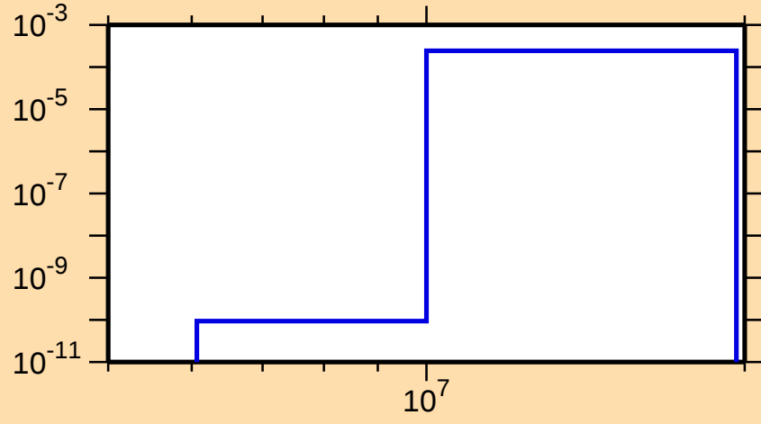
\sigma vs. E for ^{157}\text{Yb}(n,t)
