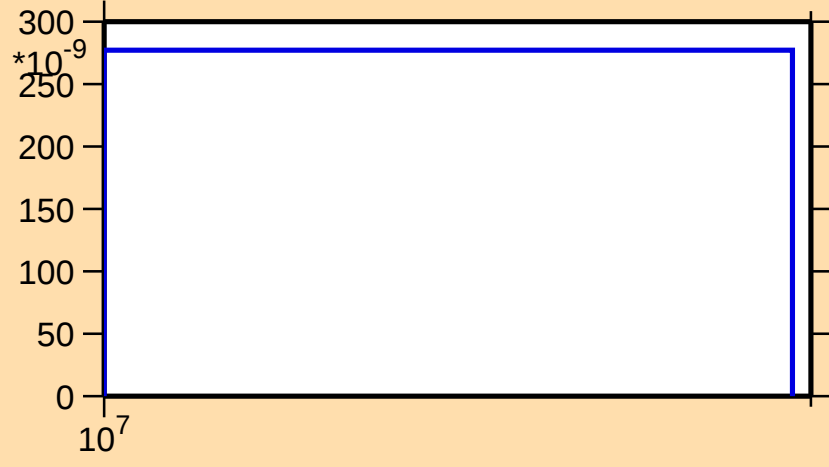
\sigma vs. E for ^{157}\text{Yb}(n,\text{nd})
