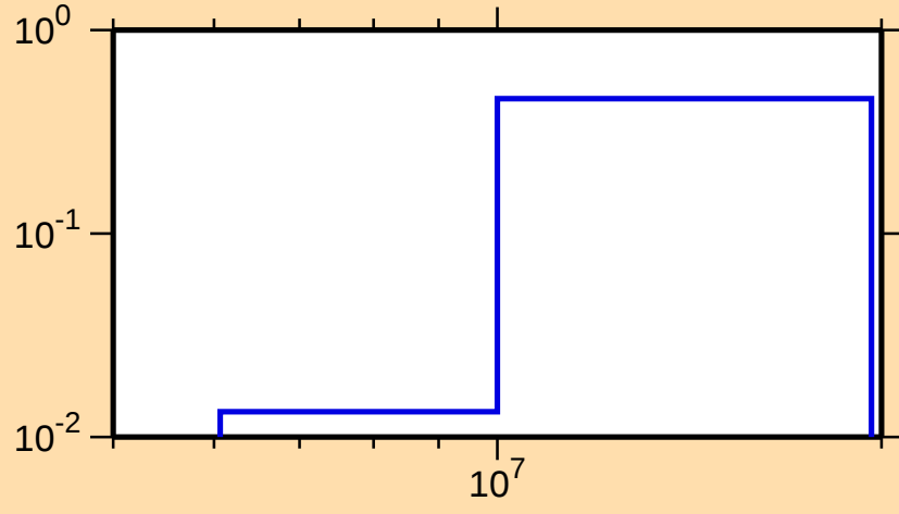
\sigma vs. E for ^{157}\text{Yb}(n,2n)
