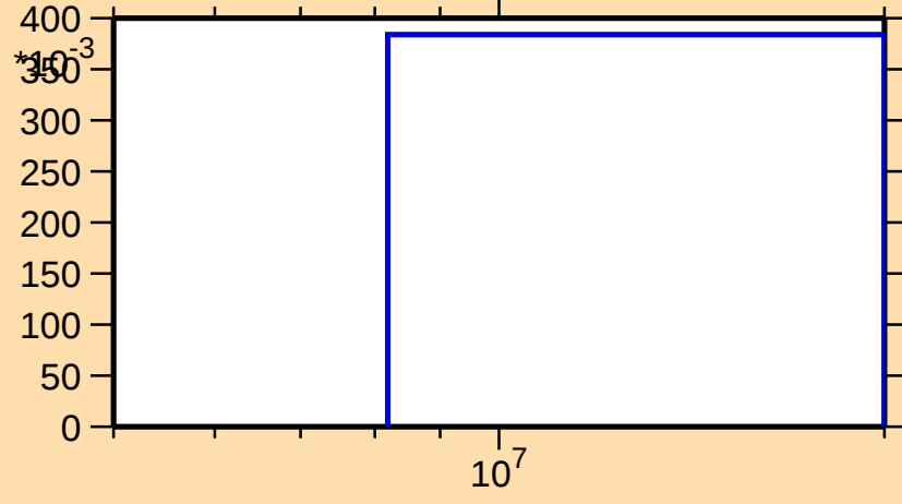
\sigma vs. E for ^{157}\text{Yb}(n,2n)
