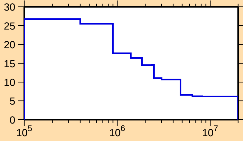
\Delta\sigma/\sigma vs. E for ^{157}\text{Yb}(n,\text{nonel.})
