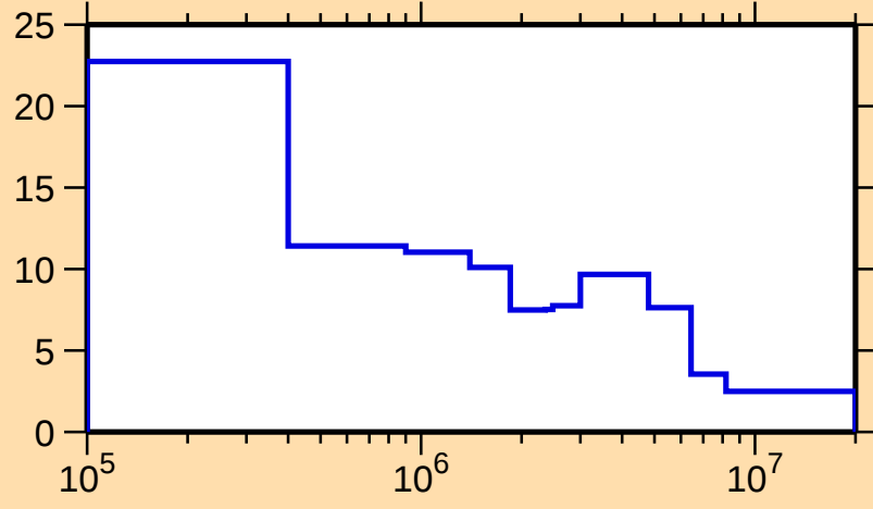
\Delta\sigma/\sigma vs. E for ^{157}\text{Yb}(n,\text{tot.})
