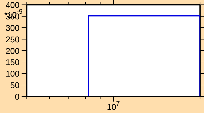
\sigma vs. E for ^{157}\text{Yb}(n,\text{pd})
