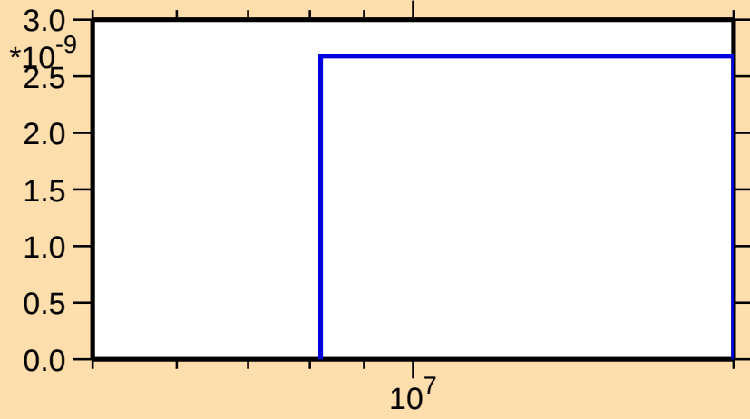
\sigma vs. E for ^{157}\text{Yb}(\text{mt117})
