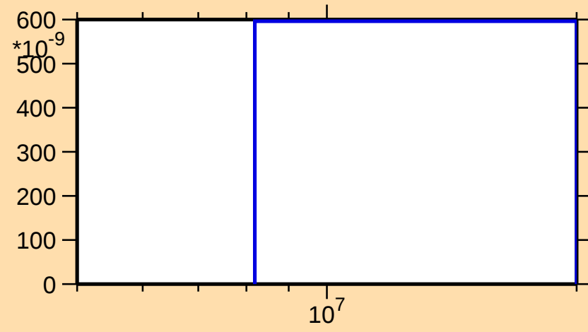
\sigma vs. E for ^{157}\text{Yb} (mt 45)
