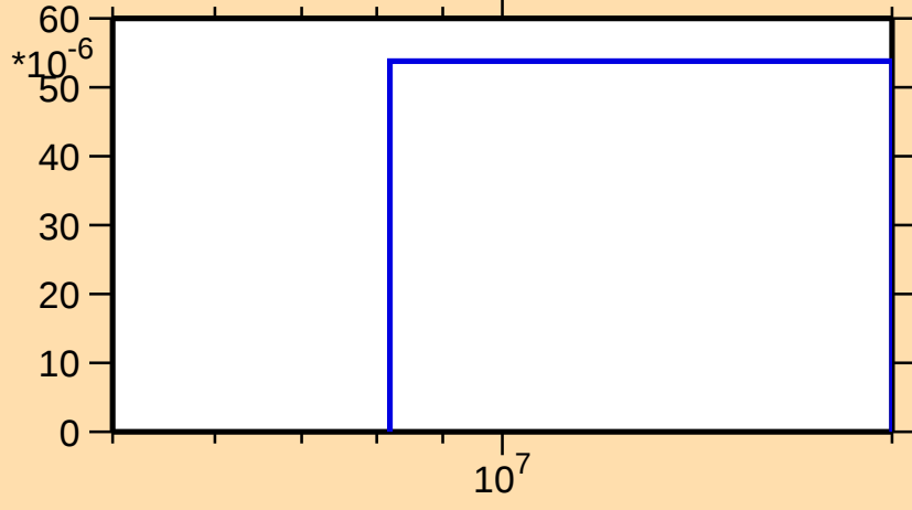
\sigma vs. E for ^{157}\text{Yb}(n,2np)
